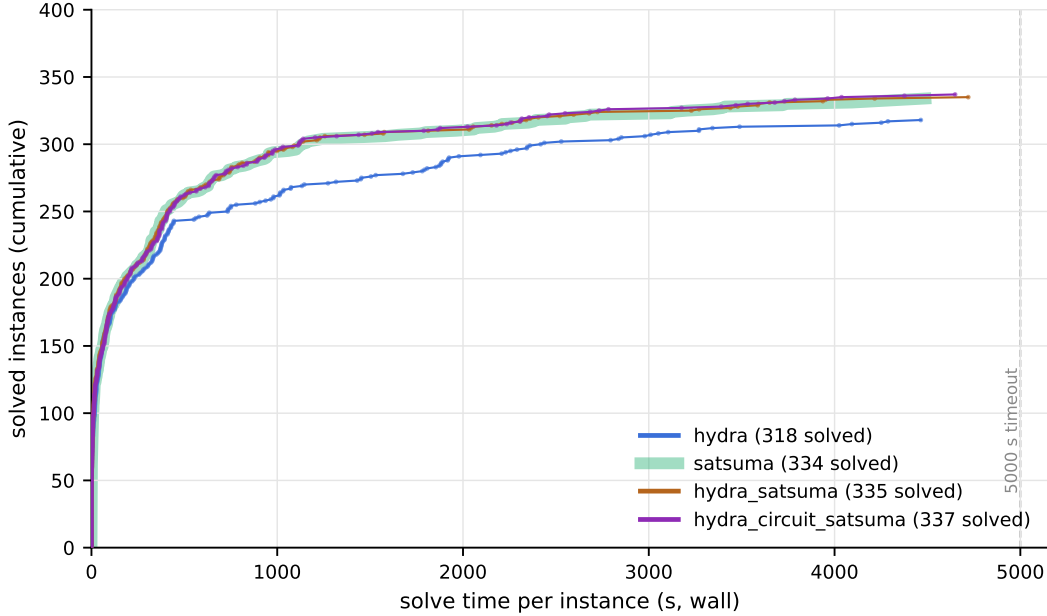
Figure 1: Cactus plot on the official 400-benchmark set: cumulative instances solved within a given per-instance time budget; one dot per solved instance, every arm aligned to the official benchmarks per hash. satsuma is drawn as a wide translucent band beneath hydra_satsuma ’s thin line because the two curves coincide almost everywhere — that near-total overlap is itself the finding (§5.1): with a symmetry-capable engine, the structural front-end changes the curve only at the chessboard pair, while the engine swap separates both from hydra from \sim 250 instances on. hydra_circuit_satsuma runs along hydra_satsuma and leaves it only at its two multiplier refutations, 1,789 and 2,308 s (§5.3); it includes the factoring stage, whose two dots sit under 0.2 s.
