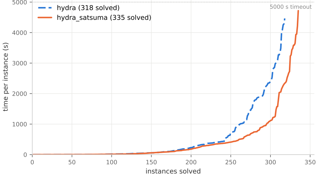
Figure 1: Cactus plot on the official 400-slot set (5000 s, certified mode, this machine): instances solved (sorted by solve time) against per-instance time. hydra is projected onto the 400 official slots per hash. The separation from \sim 250 instances on is the satsuma-iter+kissat fall-through’s contribution; the bare satsuma curve will be added when its run completes.
