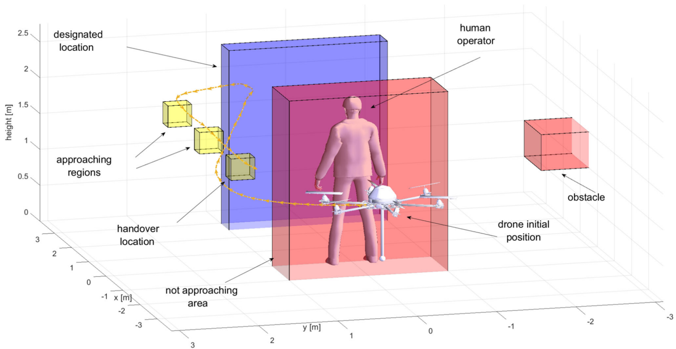
Fig. 10 Planned trajectory for the MRAV, showing a left-handed, top-to-bottom preferred approach direction, with the energy term excluded from the optimization problem (i.e., setting w = 0 in Eq. 11). Arrows indicate the paths followed by the MRAV throughout the mission
