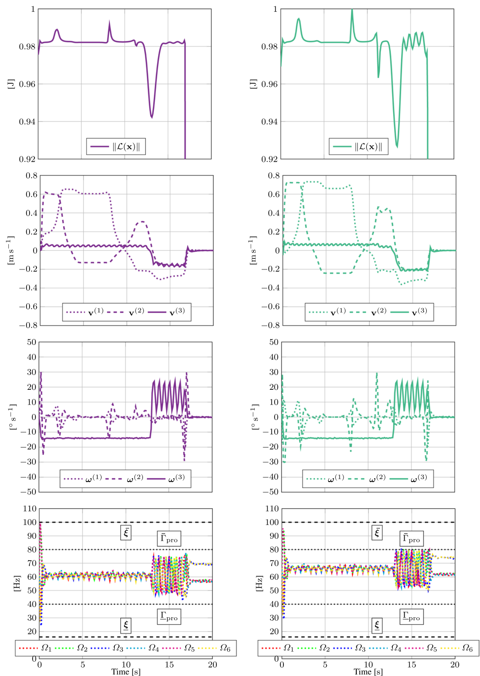
Fig. 11 Comparison of the normalized energy term, MRV linear and angular velocities, and propeller speed for scenarios where the energy term is either included (left) or excluded (right) in the optimization problem (11)
