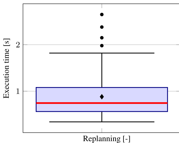
Fig. 13 Distribution of online replanning execution times over 50 runs under varying environmental perturbations. The blue box denotes the interquartile range, the red line indicates the median, and whiskers extend to the non-outlier extrema. Black dots mark outlier executions
