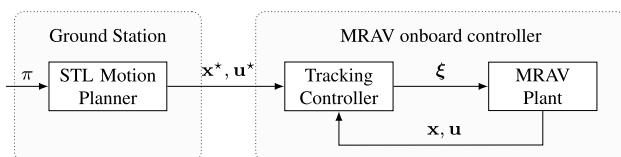
Fig. 6 System Architecture: The STL Motion Planner at the ground station generates optimal trajectories (\mathbf{x}^*, \mathbf{u}^*) for the MRAV. These trajectories are then fed into the Tracking Controller , which operates in closed loop to compute the motor forces \xi , ensuring precise flight maneuvers
