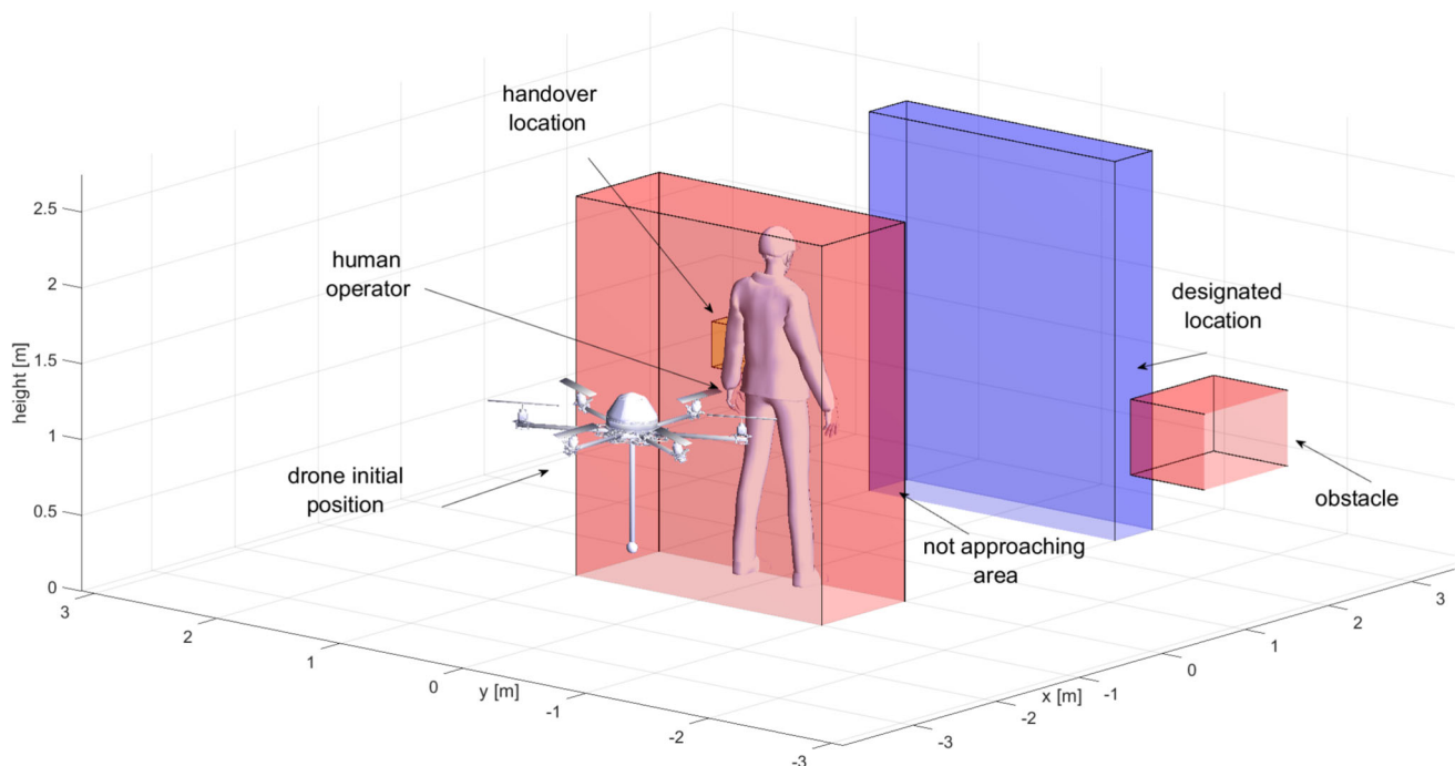
Fig. 2 Schematic depiction of the object handover scenario, highlighting the operator’s preferred handover region (yellow), the designated location (blue), and obstacles along with the restricted area behind the operator (red)
