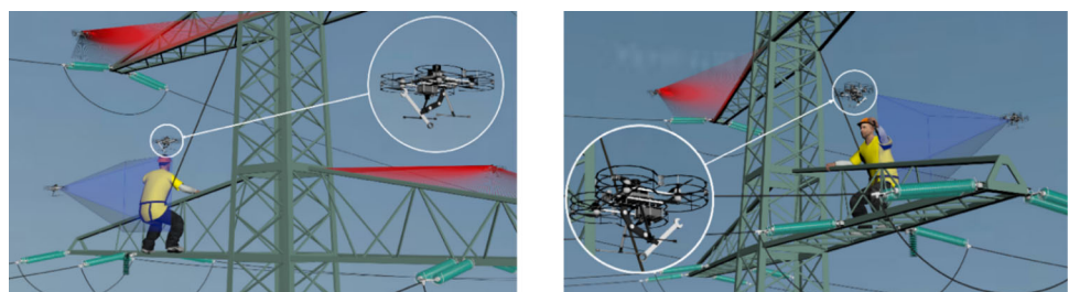
Fig. 1 Illustration of an MRV facilitating tool delivery to a human worker in a power line scenario. Courtesy of the AERIAL-CORE project 1
