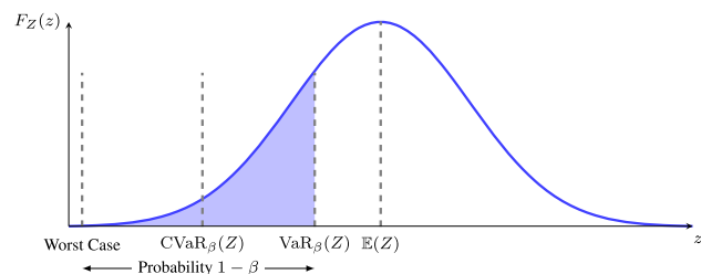
Fig. 4 Illustration of the expected value \mathbb{E}(Z) , \beta -Value-at-Risk \text{VaR}_\beta(Z) , and Conditional \beta -Value-at-Risk \text{CVaR}_\beta(Z) for a specified risk level \beta \in (0, 1) . The axes represent the stochastic variable z and its CDF F_Z(z) . The shaded area corresponds to \% \beta of the total area under F_Z(z) . \text{VaR}_\beta(Z) represents the value of z at the \beta -tail of the distribution, while \text{CVaR}_\beta(Z) averages the worst-case values of z in the \beta -tail. A negative \text{CVaR}_\beta(Z) indicates unsafe behavior
