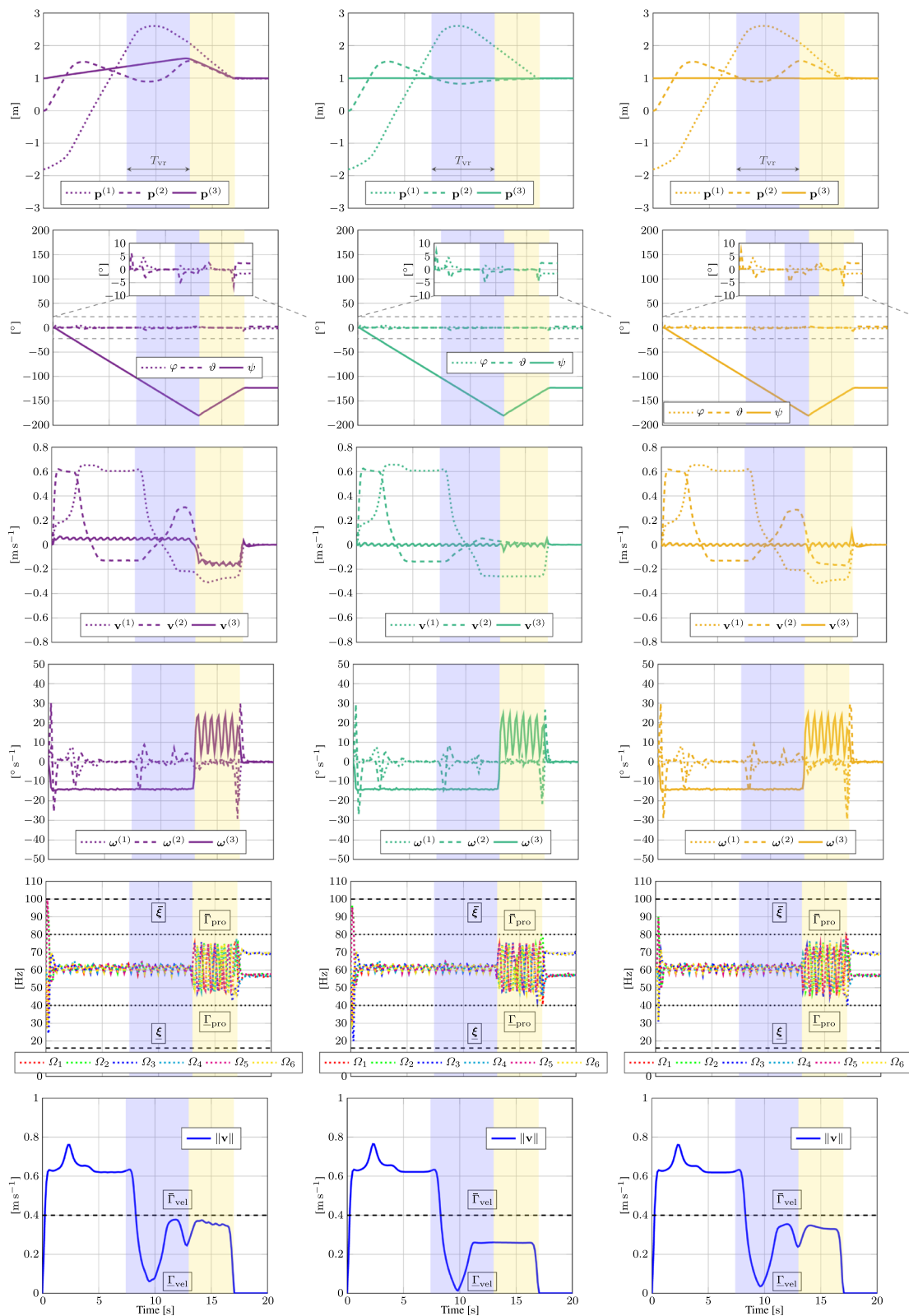
Fig. 9 Position, orientation, linear and angular velocities, propeller speed, and velocity magnitude for the planned trajectories based on different operator approach preferences: left-handed top-to-bottom
