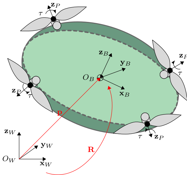
Fig. 3 Schematic representation of a GTMR system with its world \mathcal{F}_W = \{O_W, \mathbf{x}_W, \mathbf{y}_W, \mathbf{z}_W\} and body \mathcal{F}_B = \{O_B, \mathbf{x}_B, \mathbf{y}_B, \mathbf{z}_B\} reference frames
