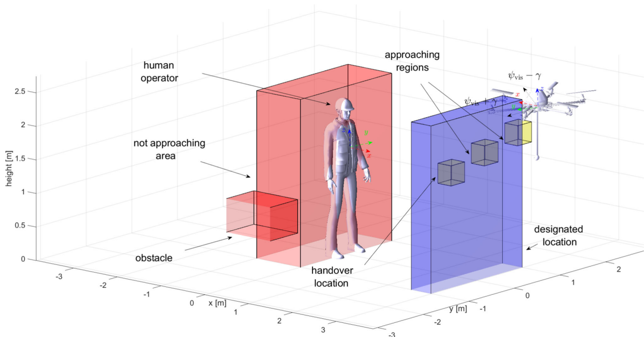
Fig. 5 Object handover scenario with highlighted approaching regions (yellow) representing the ergonomic preferences from top-to-bottom and left-to-right. Reference axes aid in visualizing the drone's maneuverability margin ( \psi_{\text{vis}} \pm \gamma ) in the displacement direction
