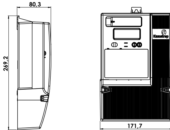
Figure 2: Dimensional sketch of OMNIPOWER CT and three-phase meter with/without breaker.
