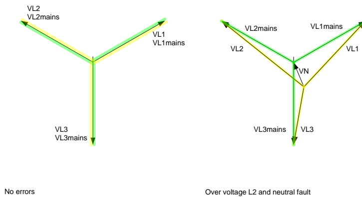
Figure 29: Neutral fault measurement principle.
