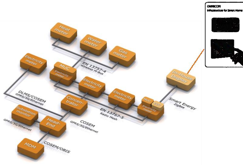
Figure 18: CCC-module in OMNIA Suite.
