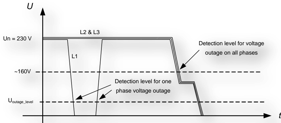
Figure 24: Detection levels for one phase and three phase voltage outage.
