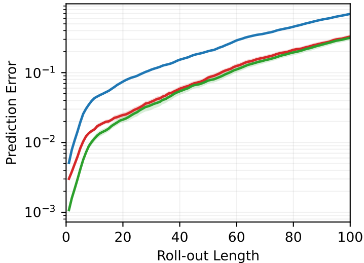
hopper-medium-replay
