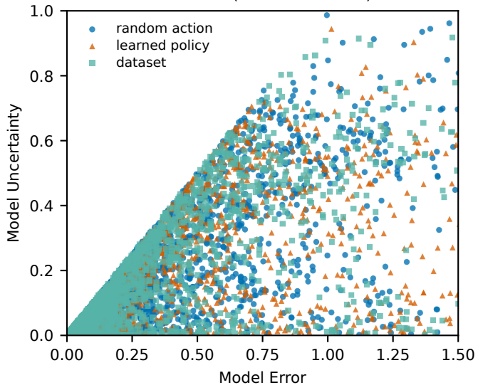
Ensemble (Correlation: 0.65)
