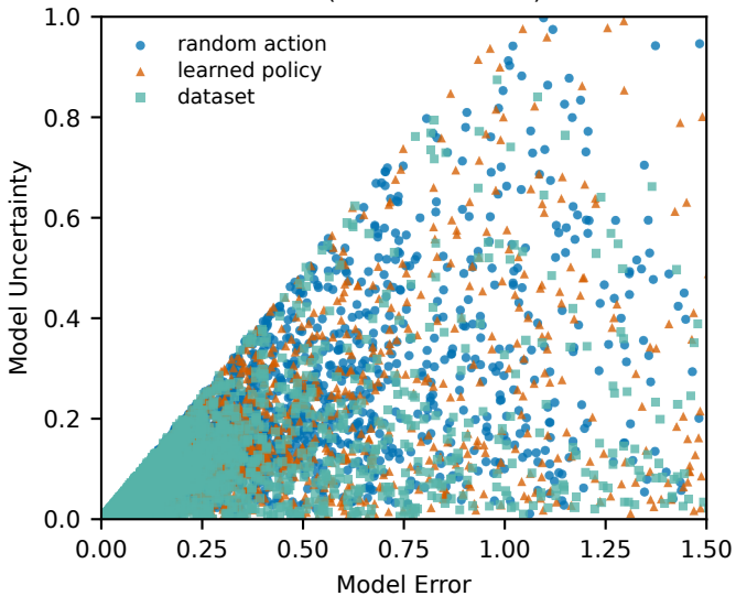
ADM (Correlation: 0.64)
