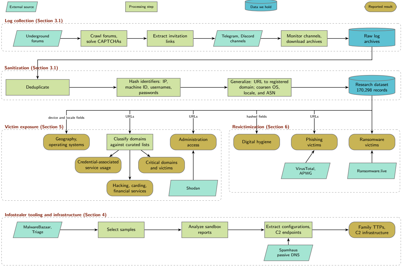
Figure 1: Pipeline of our methodology, from acquiring malware logs from illicit sources to the analyses each section reports.
