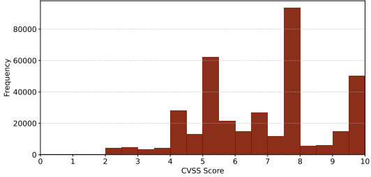
Figure 8: CVSS distribution of vulnerabilities.
