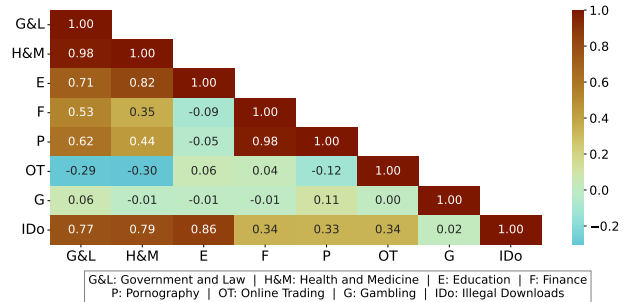
Figure 6: Cosine similarity between the categories of credential-associated service usage, under strict filtering ( > 500 domains per victim, \geq 200 victims per category; n = 322 victims).
