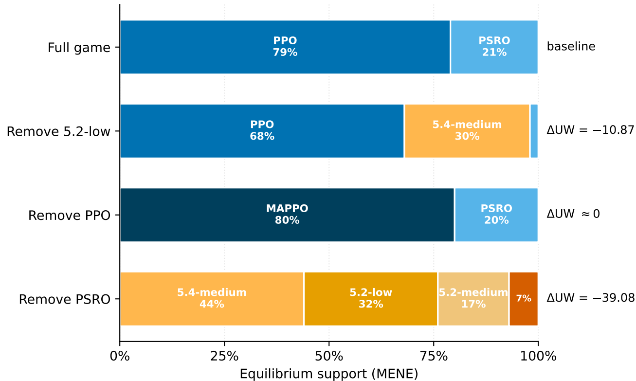
(a) Equilibrium regime shift under strategy removal
