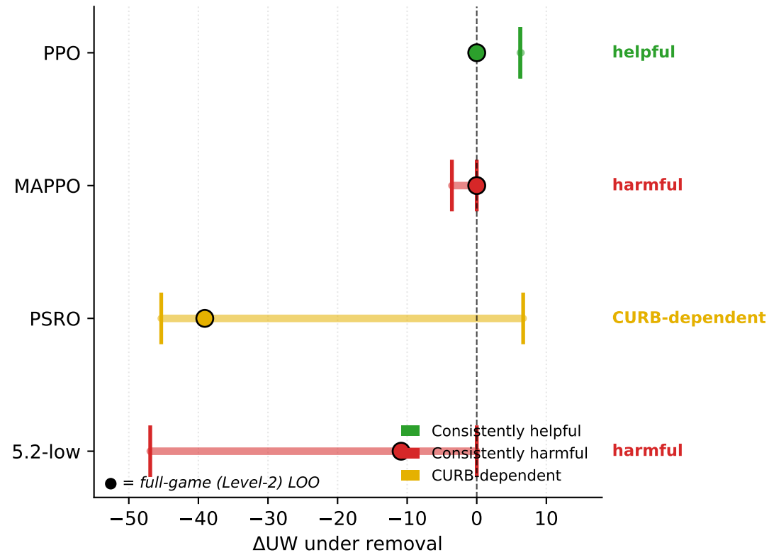
(b) Level-3 CURB-conditional LOO (UW)
