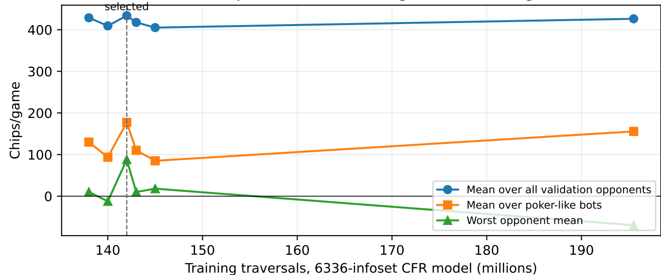
Checkpoint selection during MCCFR training
