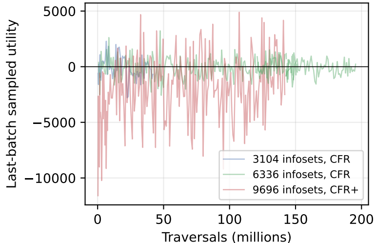
(b) Noisy self-play signal
