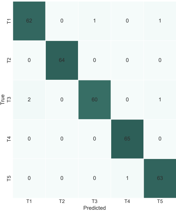
(c) CARL + SVM-RBF tuned (98.1%)
