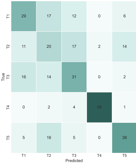
(a) HC + LDA (55.0%)
