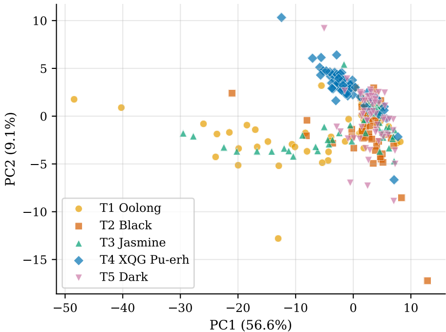
PCA of single-tea sensor responses
