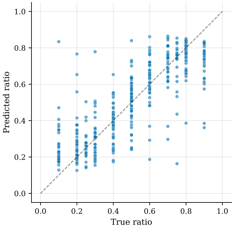
DeepMLP (CARL+combo) R^2=0.654 , MAE=0.1025
