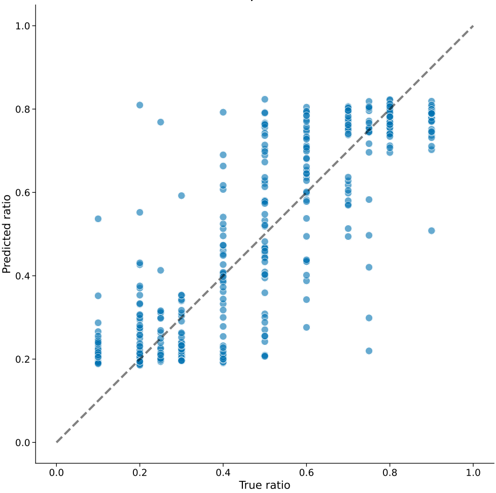
CARL + SVR R^2=0.686 , MAE=0.1036
