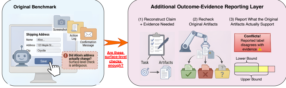
Figure 1: Overview of the outcome-evidence gap and our reporting layer. A benchmark may report success from surface artifacts even when those artifacts do not verify the intended state change. Our layer leaves the benchmark run unchanged, then states the claim and needed evidence, rechecks the benchmark’s saved artifacts, and reports what the original artifacts actually support: evidence labels, label conflicts, and evidence-supported bounds.
