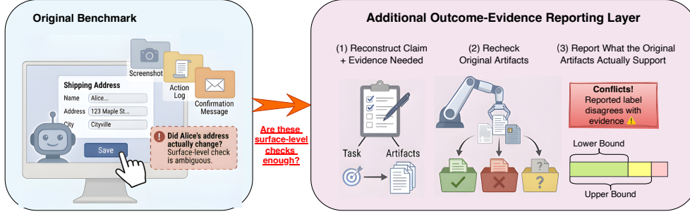
Figure 1: Overview of the outcome-evidence gap and our reporting layer. A benchmark can report success from surface artifacts even when those artifacts do not verify the intended state change. Our layer leaves the benchmark run unchanged, then states the claim and needed evidence, rechecks the benchmark’s saved artifacts, and reports what the original artifacts support: evidence labels, benchmark conflicts, and evidence-supported bounds.
