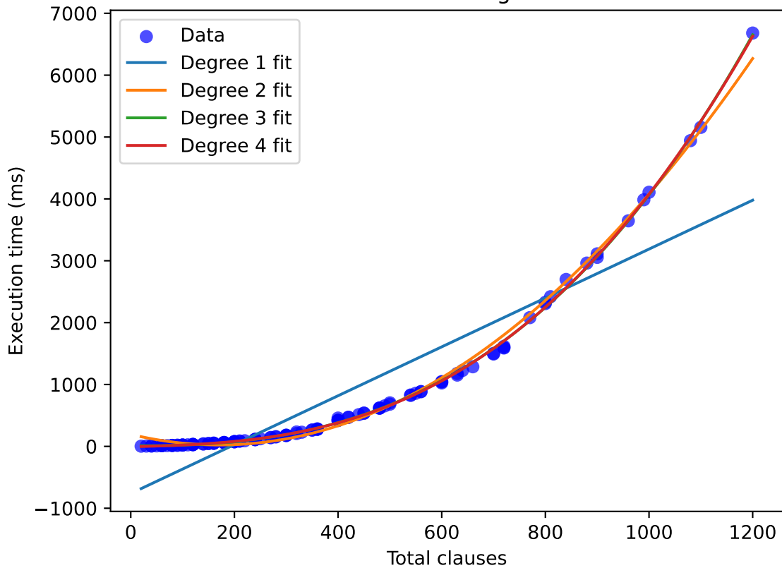
Data fitting
