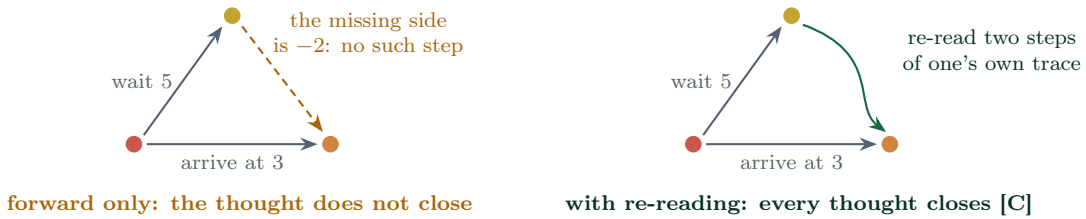
Figure 10: The bridge that needs a backward plank. Two thoughts of different lengths ask to be closed by a third; over bare forward time the closing side would have to be negative, and the composition refuses — on the census grid, 42.9% of all posable closures. Re-reading one’s own trace supplies the lawful negative step: the world does not rewind — the knowledge does [C].
