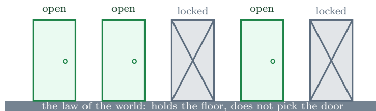
Figure 10: Freedom in UHM is not the law’s suspension but its silence along part of the directions. It is computable in every state, differs between states, and responds to training: learning literally opens doors .
