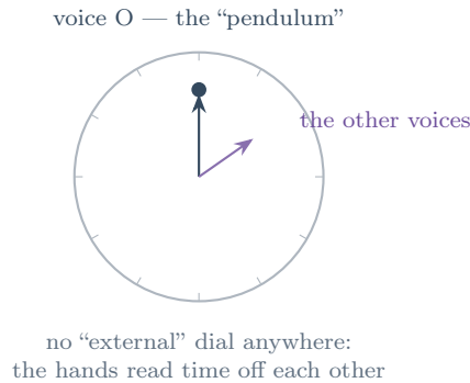
Figure 2: Time in UHM: not a river the world floats in, but the mutual attunement of the world’s parts. The question “what was there when time did not yet exist” turns from a deep one into a grammatical error — like “what is north of the North Pole.”
