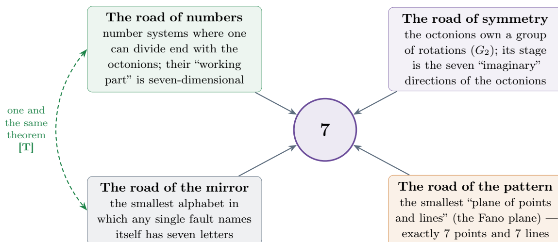
Figure 1: Four roads to seven. Especially beautiful: the road of numbers and the road of the mirror are not a coincidence but a proven identity [T] : “the last system where division works” and “the last alphabet that checks itself” are one and the same property, seen from two sides.
