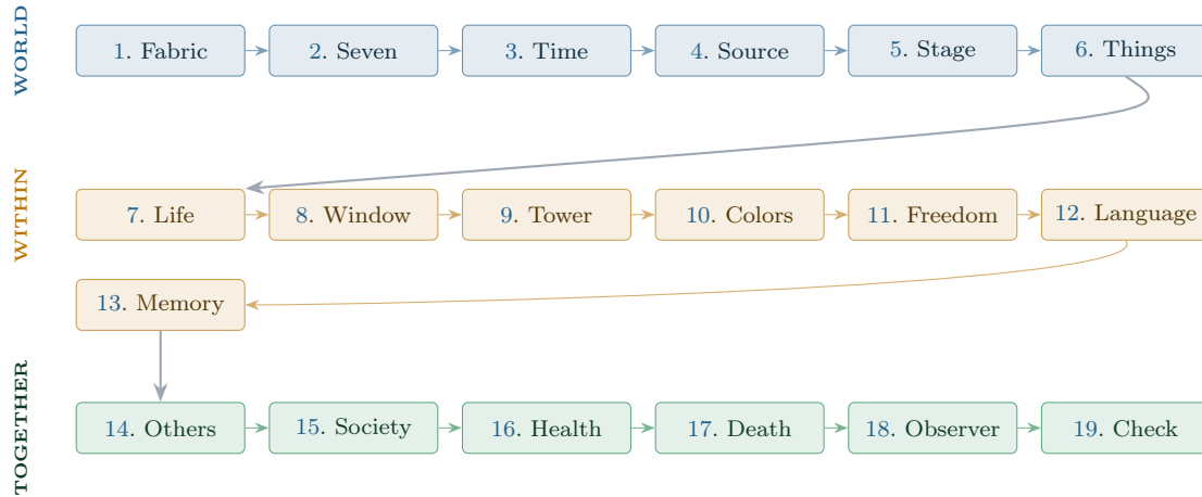
Figure 16: The map of the road: from the world’s fabric — through the birth of the inner — to living together and to the check. Each band can also be read on its own.
