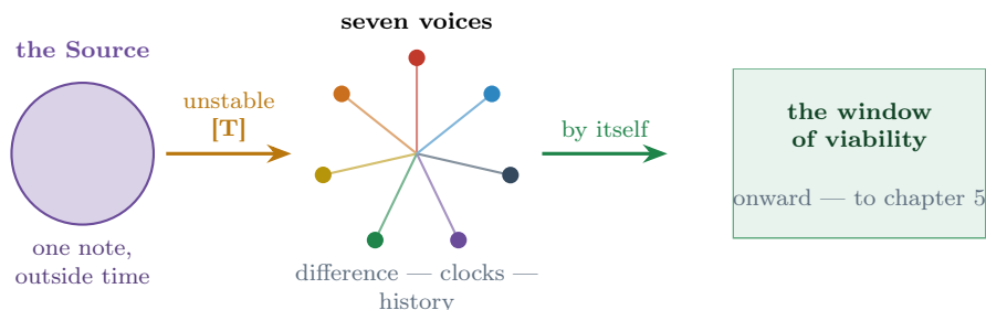
Figure 3: Cosmogenesis in UHM: the Source (postulate [P]) is unstable (theorem [T]), unlayers into seven voices with clocks and history, and slides by itself into the window of life (machine verified). The question “what was before?” is dissolved: “before” is a word born at the second step of this picture.
