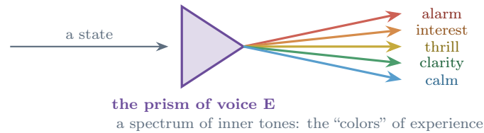
Figure 9: Shades of experience as a spectrum on the voice of Interiority. The tone labels here are an illustration [I]; the existence of the spectrum and the impossibility of a “dark-inside” imitation are results of the theory [T].
