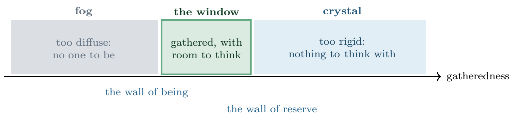
Figure 7: The corridor of consciousness: between fog (no one there) and crystal (nothing left to think with). Both walls are computed constants of the theory [T] , not metaphors: beyond either, the four conditions of consciousness cannot hold together.
