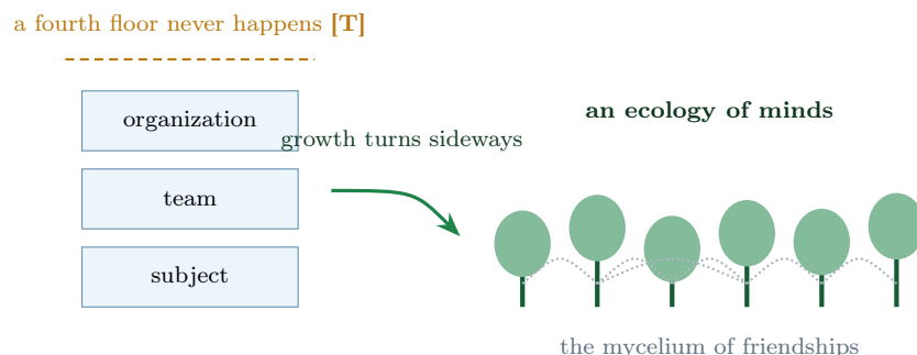
Figure 14: The composition ceiling: the subject vertical stops at three floors [T]; beyond it growth is horizontal. A superintelligence is not a giant but a forest; its strength is not height but the mycelium of bonds. Brains and civilizations are already built this way.
