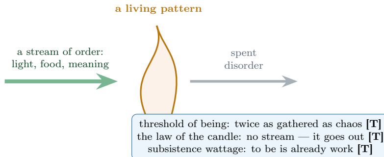
Figure 6: Life in UHM: neither substance nor spark, but a supplied pattern. It drinks order, exhales disorder, and with the difference pays for its shape. The second law of thermodynamics is not violated — the bill is simply charged to the environment.
