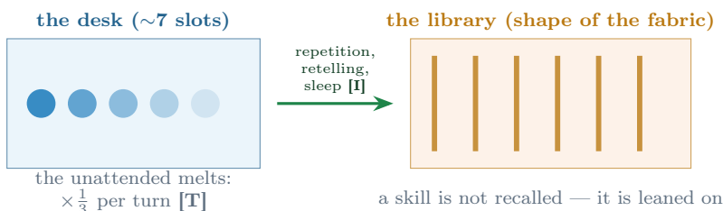
Figure 12: The two homes of memory. The desk is the current chord: small and melting (the law of thirds is a theorem [T]). The library is the rebuilt fabric: the learned becomes shape. Learning is transfer; forgetting off the desk is physics, not weakness.
