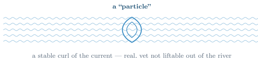
Figure 5: A particle in UHM is a pattern in the fabric of agreements, not a grain of stuff. Light patterns are the familiar particles; the lightest massive one is the lightest neutrino ( \lesssim 0.004 eV [C]); a special heavy, indestructible pattern of the voice O is the dark-matter candidate [C].
