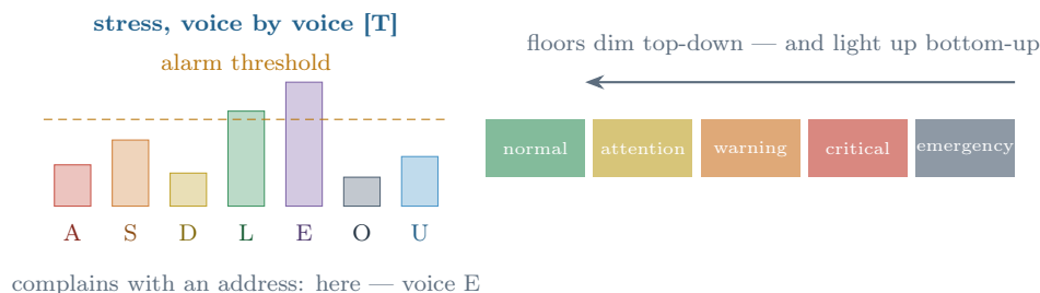
Figure 15: The instrument panel of care: addressed per-voice stress [T] and the ladder of regimes. Overload switches the upper floors of reflection off first; recovery goes in reverse order. Suffering is a measurable rate of slide — so care is flow engineering, not only compassion.
