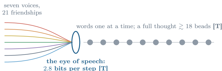
Figure 11: Language is the serial unloading of a voluminous chord through a one-dimensional eye. The narrowness of the channel is a theorem, not a metaphor: hence both the length of a “complete thought” and the very need for grammar.
