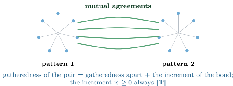
Figure 13: Cooperation in UHM: the coupling of two patterns is a strictly nonnegative increment to their joint being. Rivalry is not the “minus” of this quantity (it has no minus) but a contest over shared supply streams — a phenomenon of chapter 7, not of this one.
