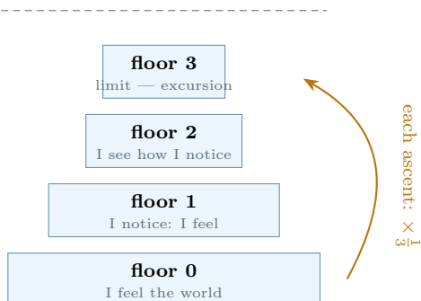
Figure 8: The tower of reflection. Each turn inward keeps one third of distinguishability; after the third turn the remainder sinks below the threshold of telling-apart — the fourth floor is structurally empty [T]. The same law limits “I know that you know that I know”: the third step is the ceiling of mutual mind-reading.
