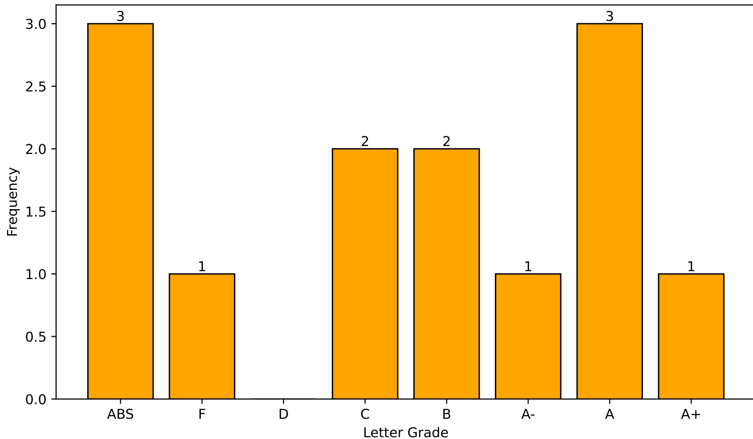
Class Letter Grade Distribution
