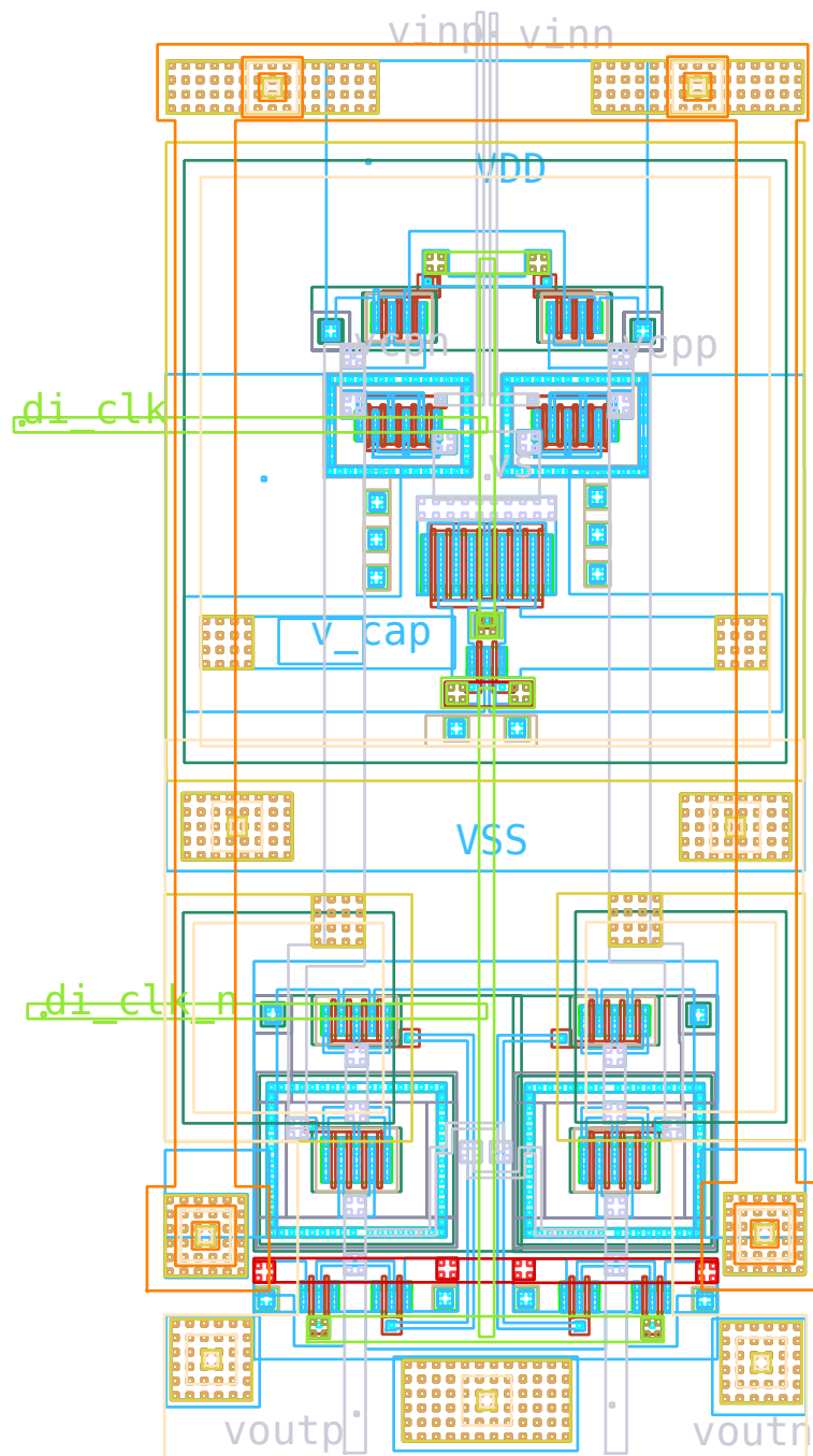
Figura 3.3: Layout Bindra
