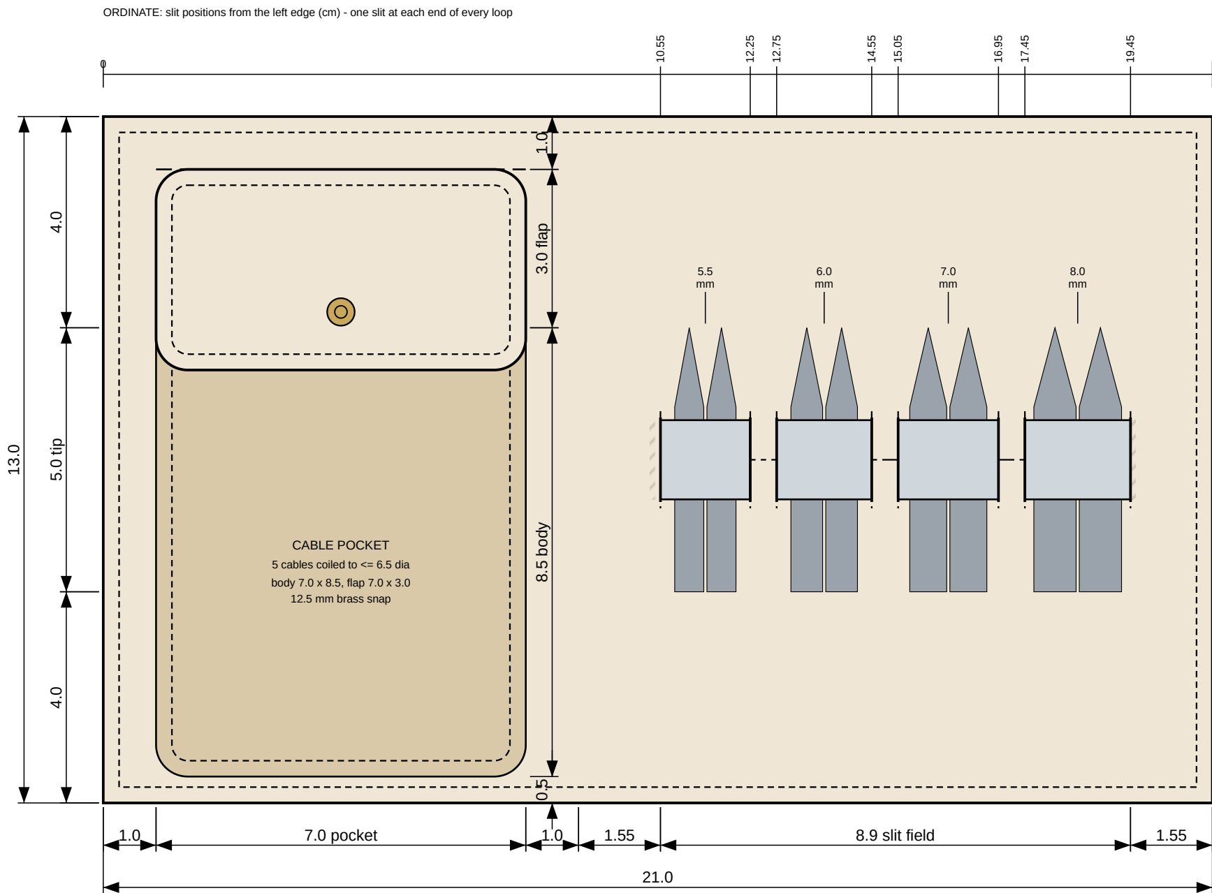
PANEL 4 - BACK-WALL LINING 21.0 x 13.0 (inner face of the back wall; not a loose page). Full size 1:1 - use as slit template.
