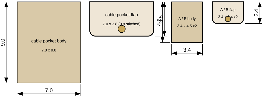
DETAIL D - POCKET PATTERNS, 1:2 (net; add 0.8 turn-under on the three stitched sides, top edge bound or skived)
