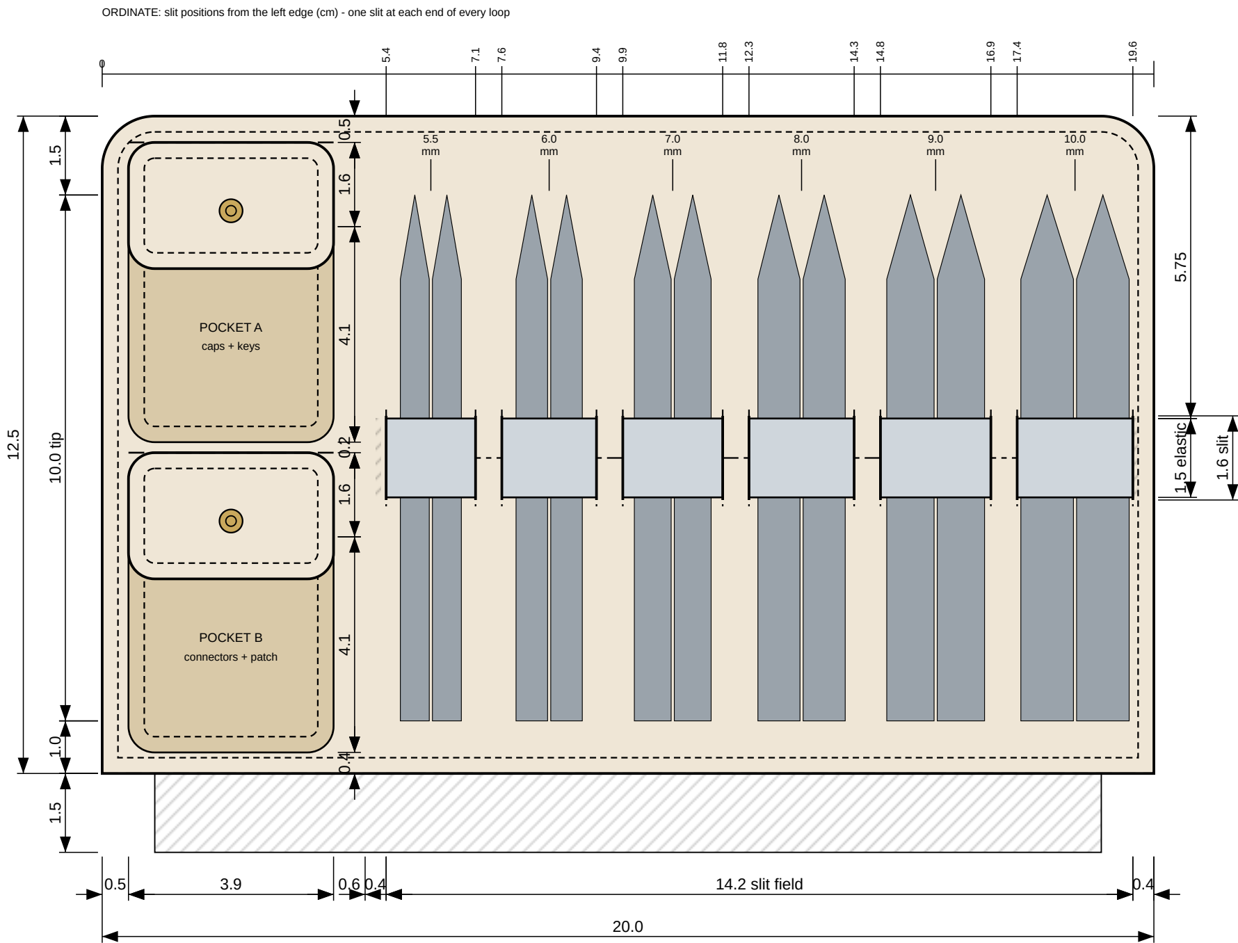
PANEL 2 - page 20.0 x 12.5 + 1.5 hinge tab. Full size 1:1 - use as slit template.
