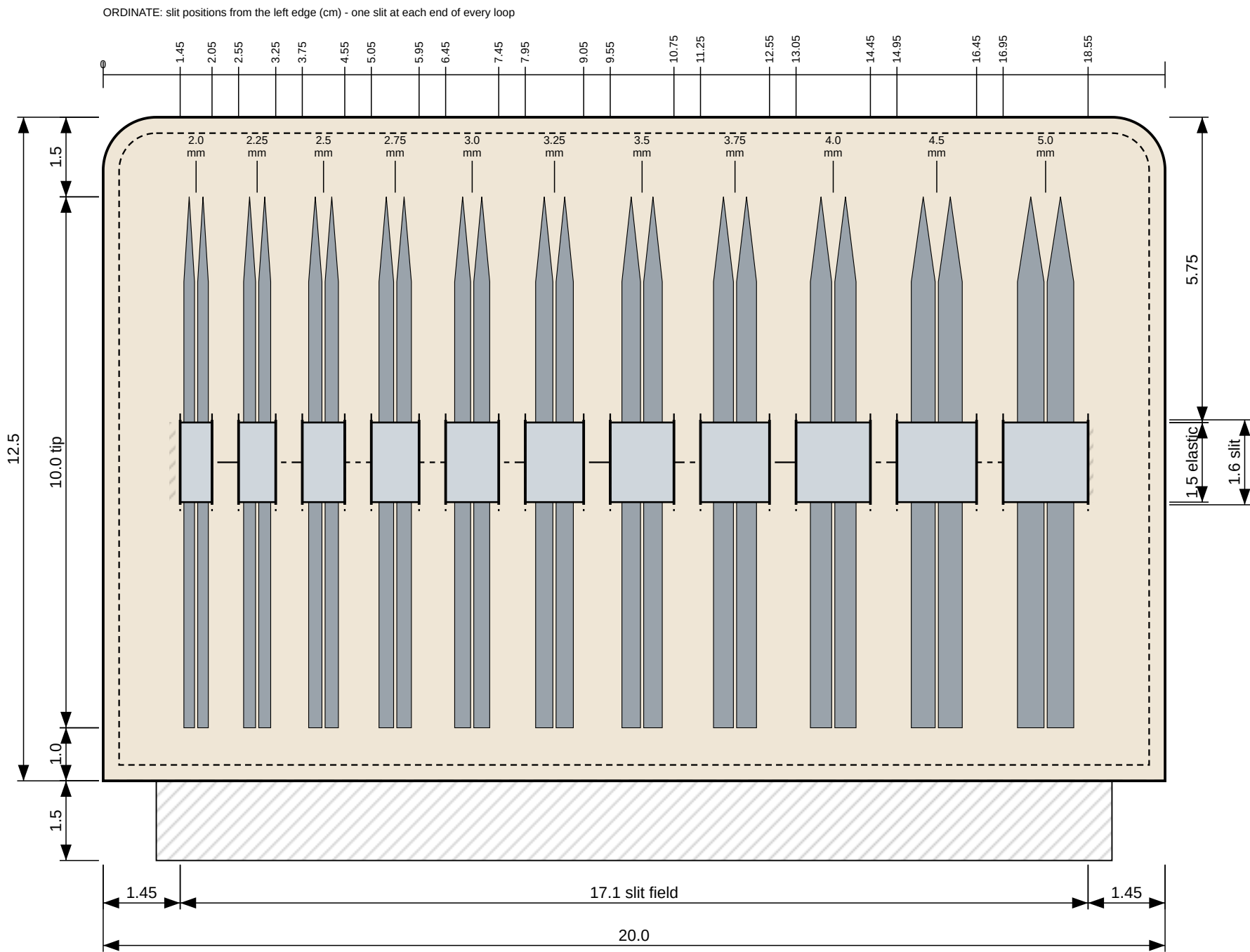
PANEL 1 (PAGE) - page 20.0 x 12.5 + 1.5 hinge tab. Full size 1:1 - use as slit template.
