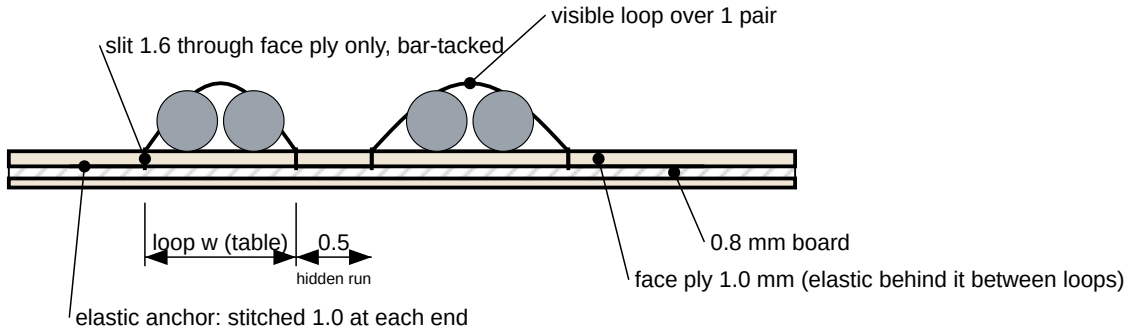
DETAIL A - elastic threaded through the face ply, section, 2:1
