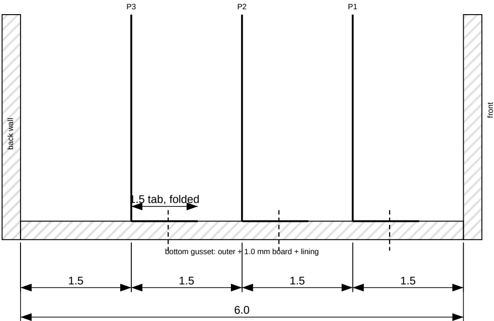
DETAIL C - PAGE HINGES, section through the bottom gusset, 2:1
