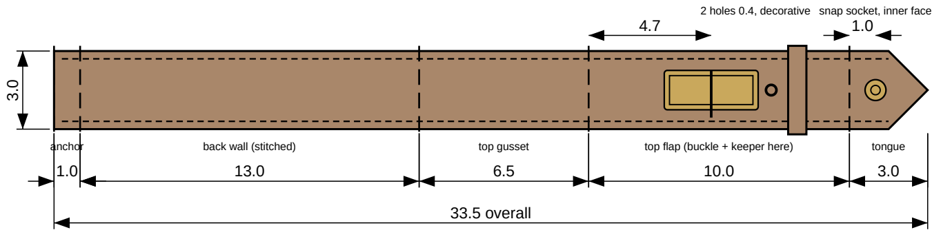
DETAIL B - STRAP, flat, 1:2 (dark brown leather 1.4 mm, 2 ply, edge-stitched 0.3)
