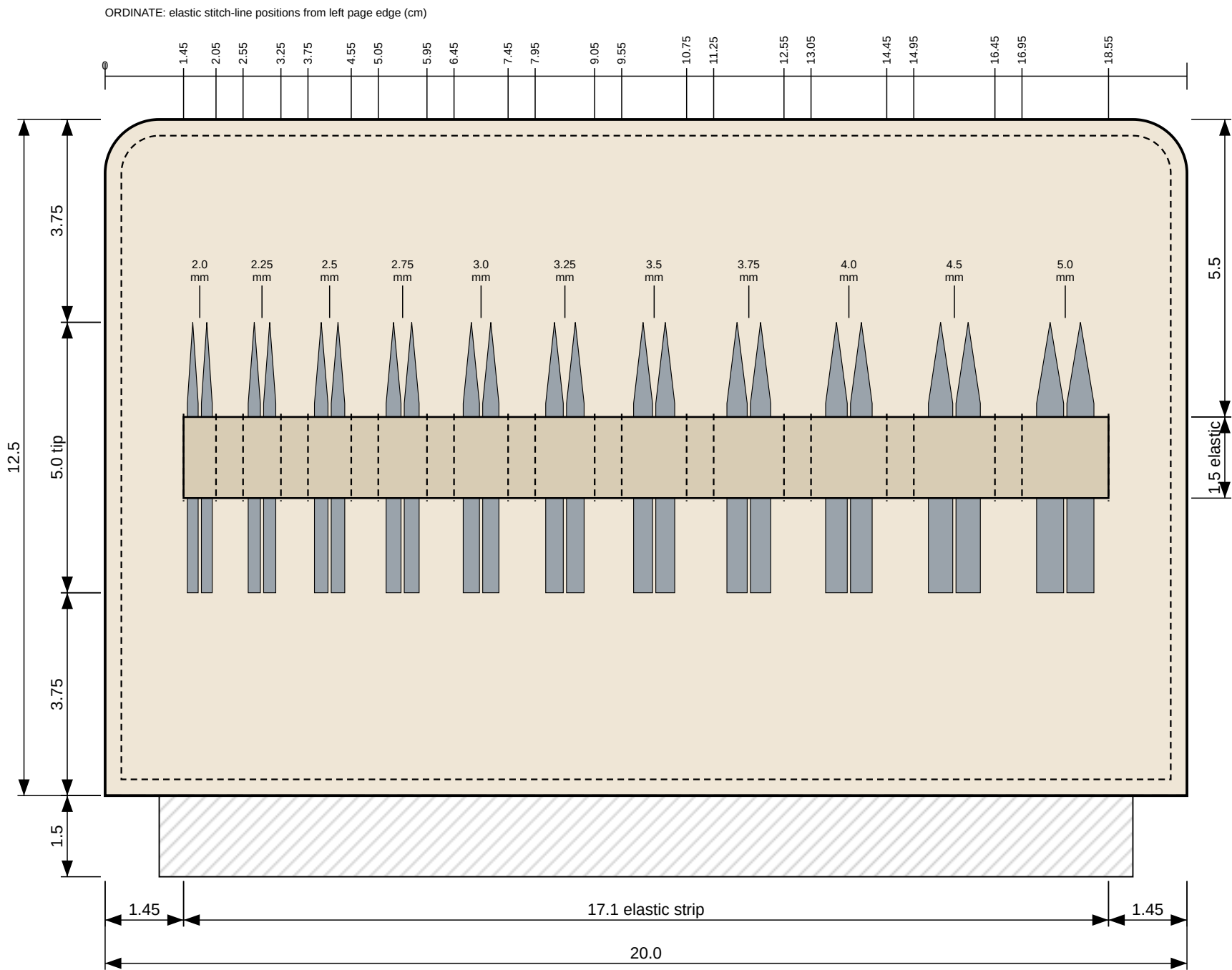
PAGE 3 - 20.0 x 12.5 + 1.5 hinge tab. Full size 1:1 - use as pattern.
