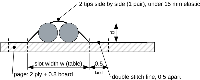
DETAIL A - elastic slot section, 2:1
