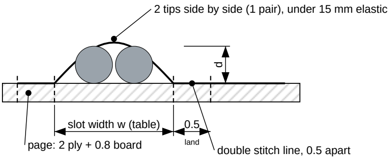
DETAIL A - elastic slot section, 2:1 (same on all pages)
