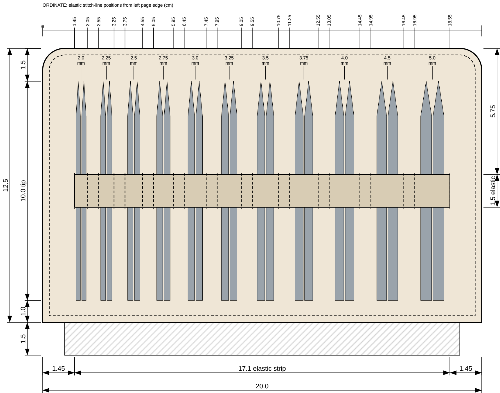
PAGE 1 - 20.0 x 12.5 + 1.5 hinge tab. Full size 1:1 - use as pattern.
