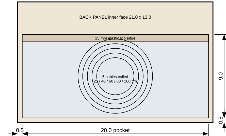
DETAIL D - CABLE POCKET on the inner face of the back panel, behind page 1 (1:2)
