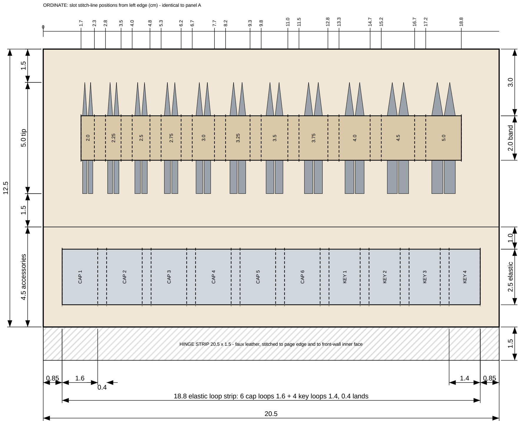
PAGE FACE 1 - 20.5 x 12.5 (page hinge along the BOTTOM edge, 1.5 cm strip to front wall). Full size 1:1 - use as pattern.
