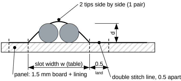
DETAIL A - slot band section, 2:1
