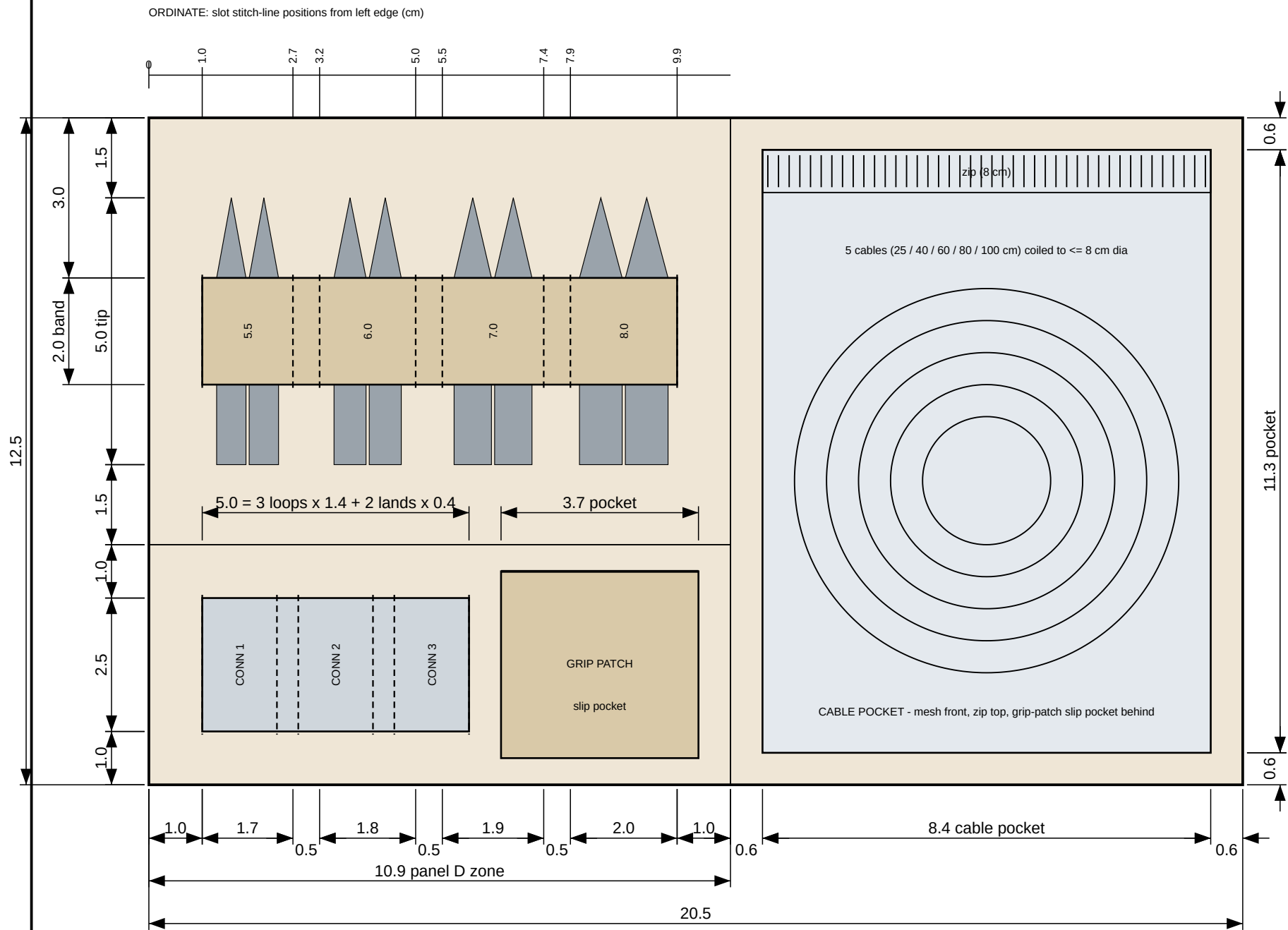
PAGE FACE 2 - 20.5 x 12.5 (reverse of face 1; hinge along the BOTTOM edge). Full size 1:1 - use as pattern.
