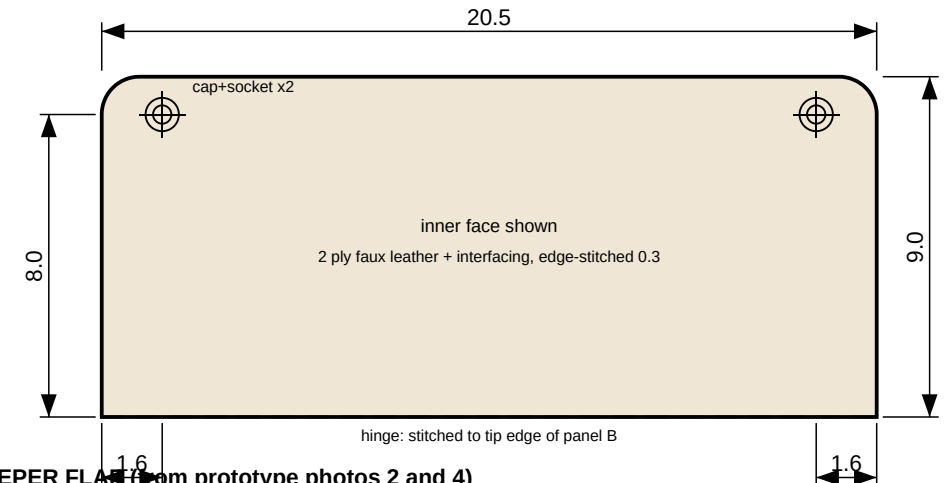
KEEPER FLAG (from prototype photos 2 and 4)
