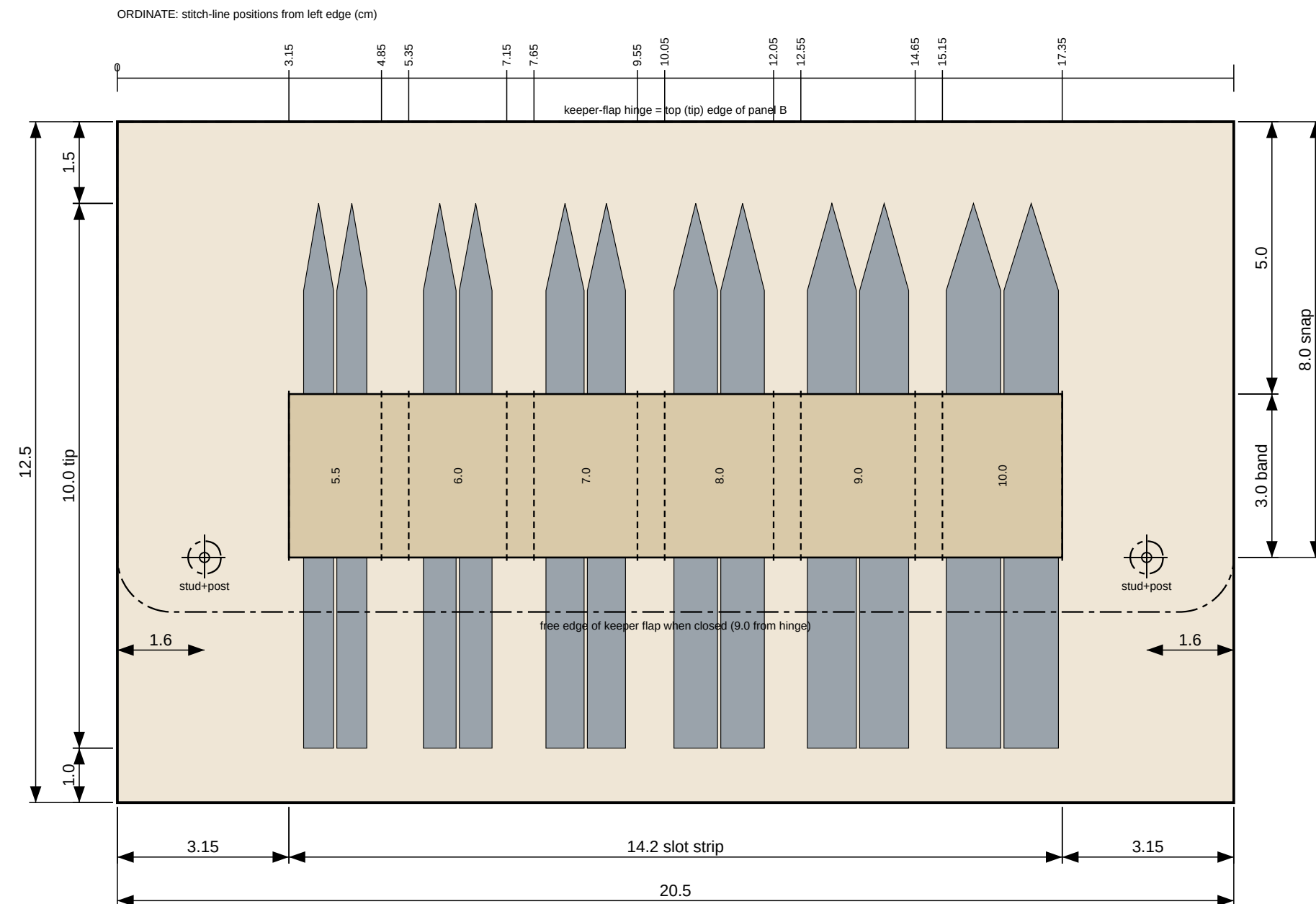
KEEPER FLAG (from prototype photos 2 and 4)
