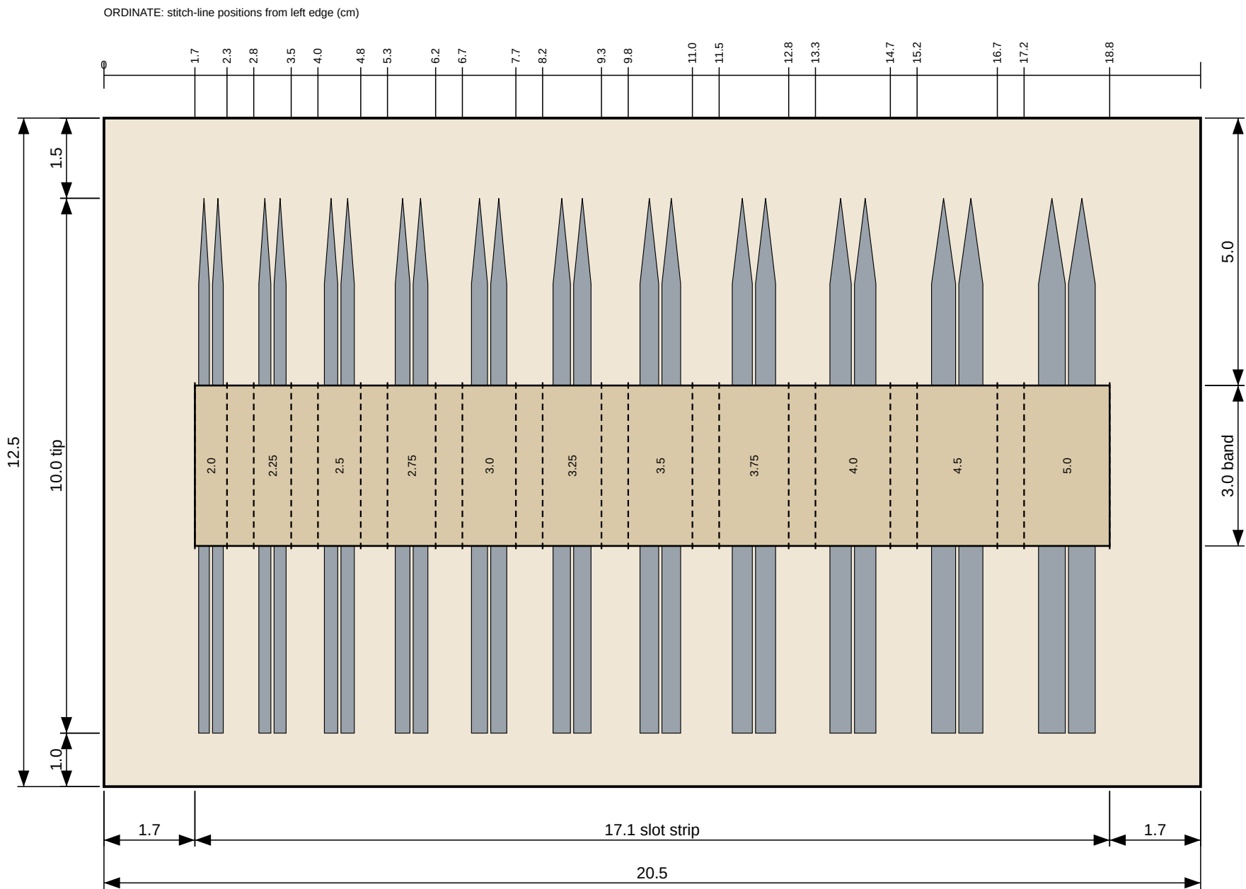
PANEL A - 20.5 x 12.5, fits BASE interior. Full size 1:1 - use as pattern.
