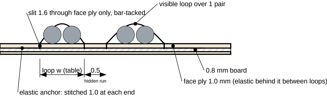
DETAIL A - elastic threaded through the face ply, section, 2:1
