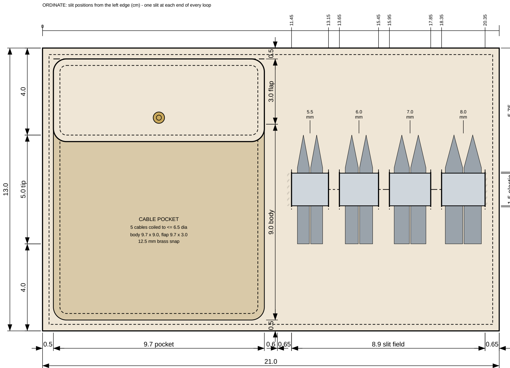
PANEL 4 - BACK-WALL LINING 21.0 x 13.0 (inner face of the back wall; not a loose page). Full size 1:1 - use as slit template.
