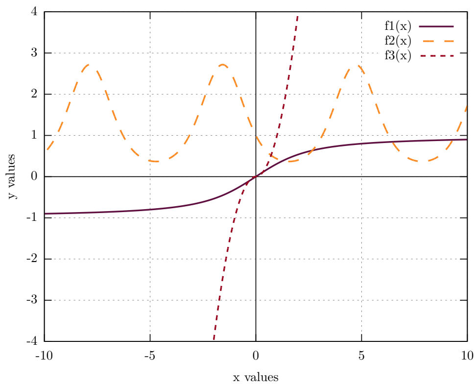
Figure 1: f_1(x) = \coth(x) - \frac{1}{x} , f_2(x) = e^{-\sin(x)} , f_3(x) = x|x|
