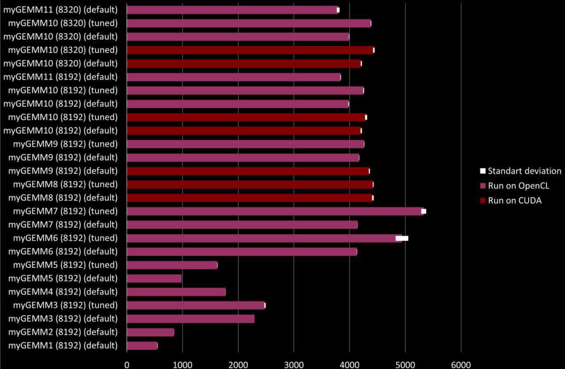
GFLOPS (8192x8192x8192 and 8320x8320x8320 on NVIDIA GeForce RTX 4060 Laptop GPU)
