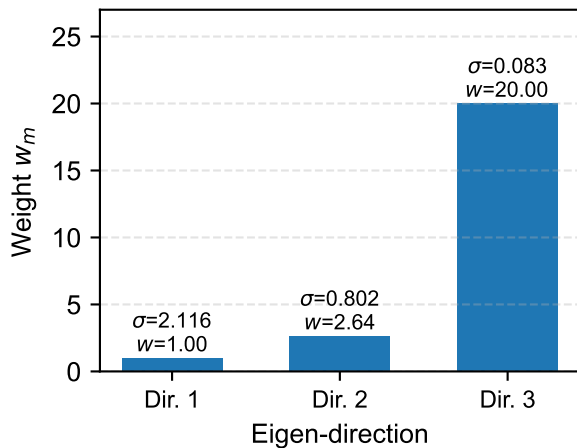
Spectral-direction weights
