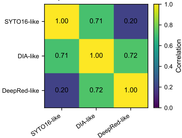
Spectral Gram matrix C
