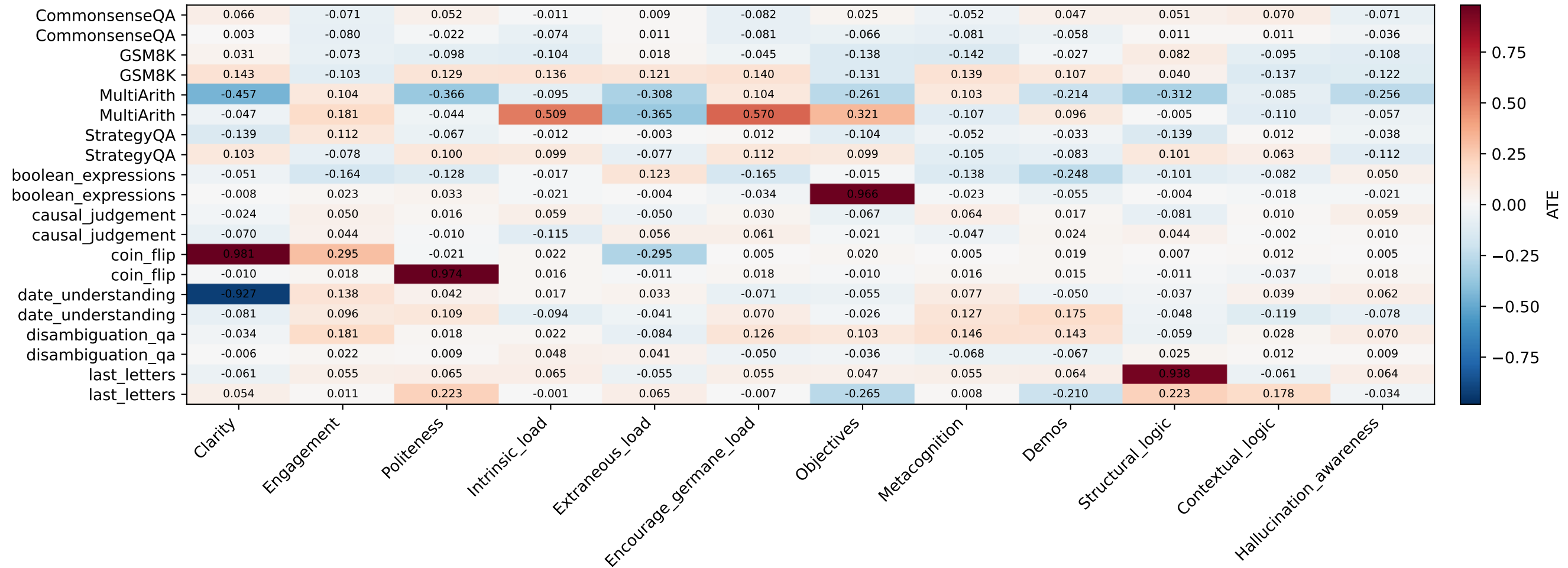
DSpy MIPROv2 ATE Heatmap (centered at 0)
