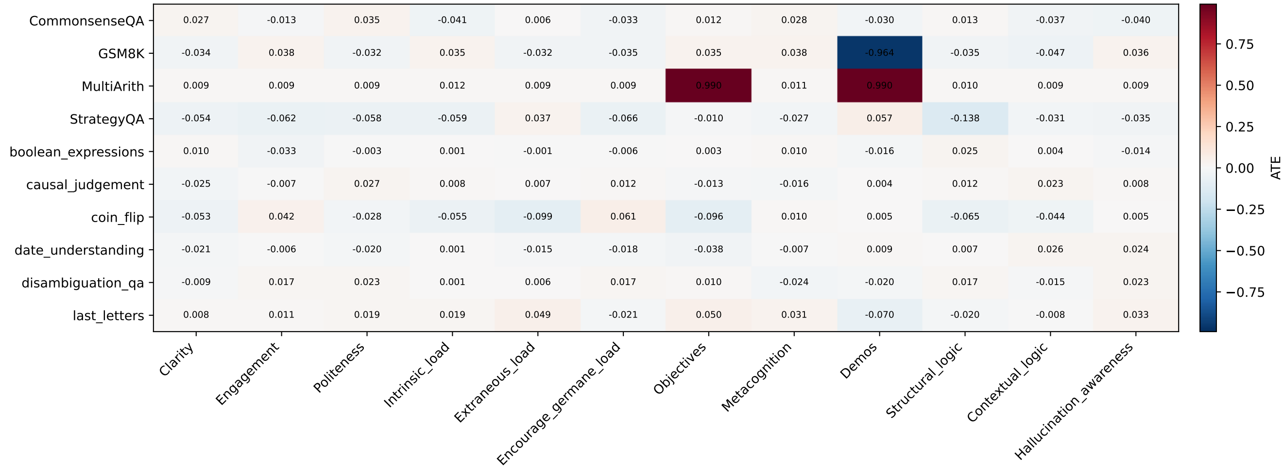
TextGrad ATE Heatmap (centered at 0)
