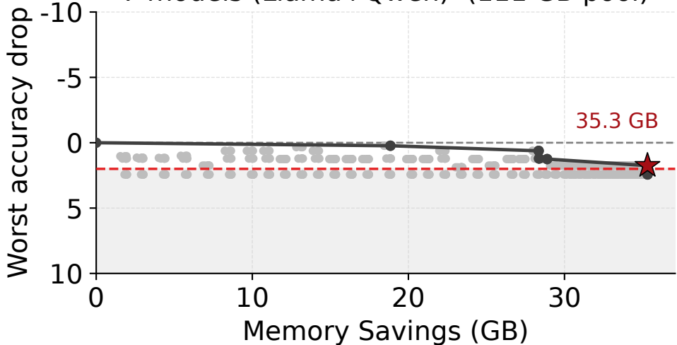
7 models (Llama+Qwen) (111 GB pool)
