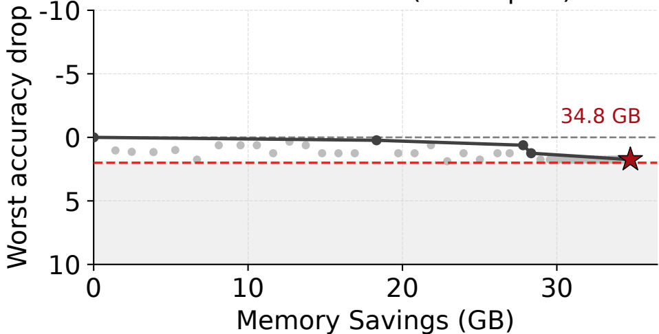
5× Llama-3.1-8B (80 GB pool)
