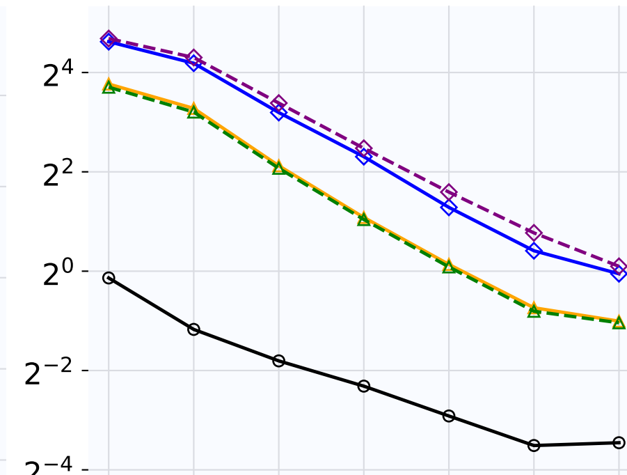
(c) GAP-twitter
