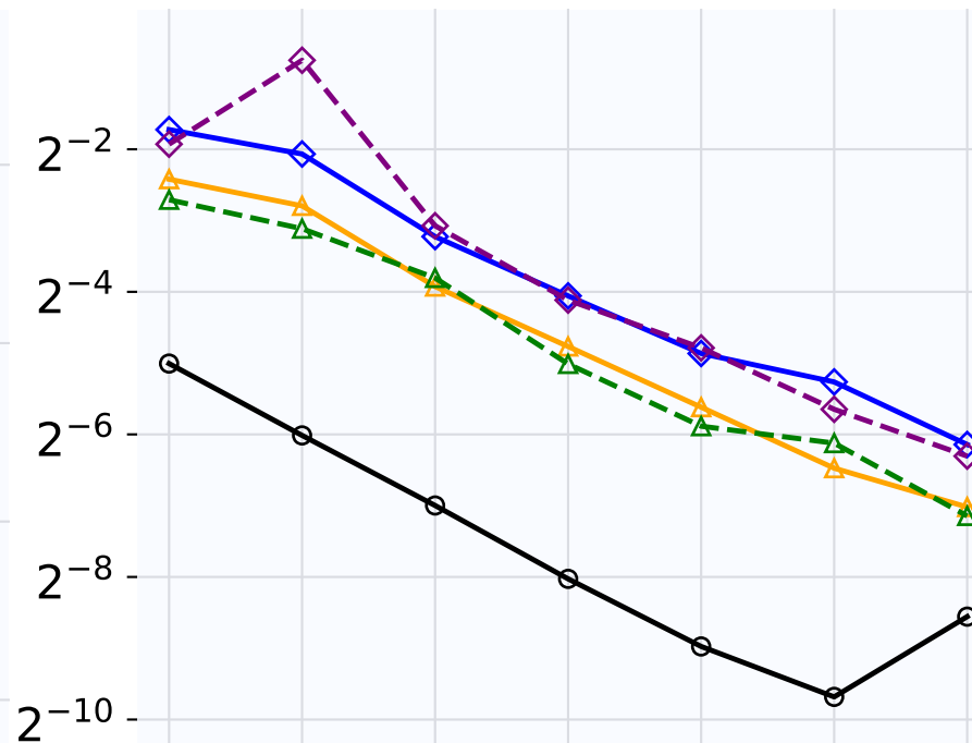
(b) GAP-road
