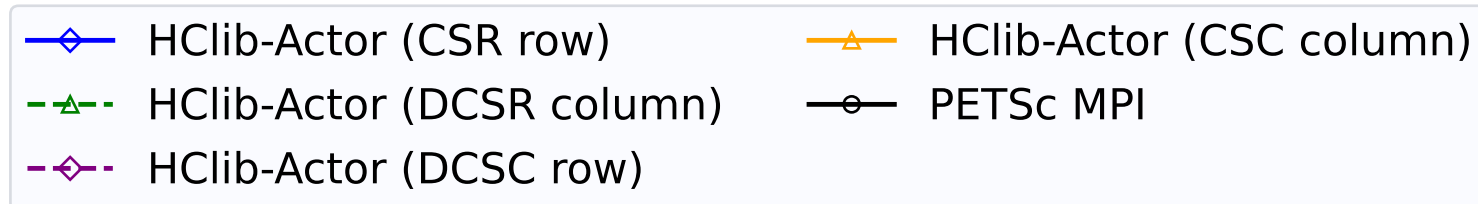
(b) GAP-road
