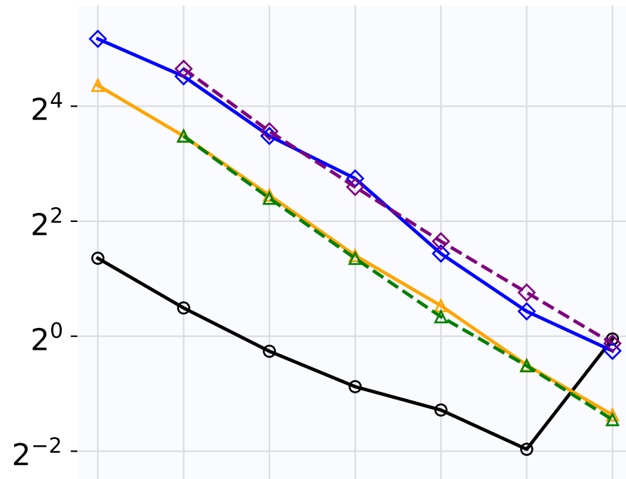
(a) GAP-kron
