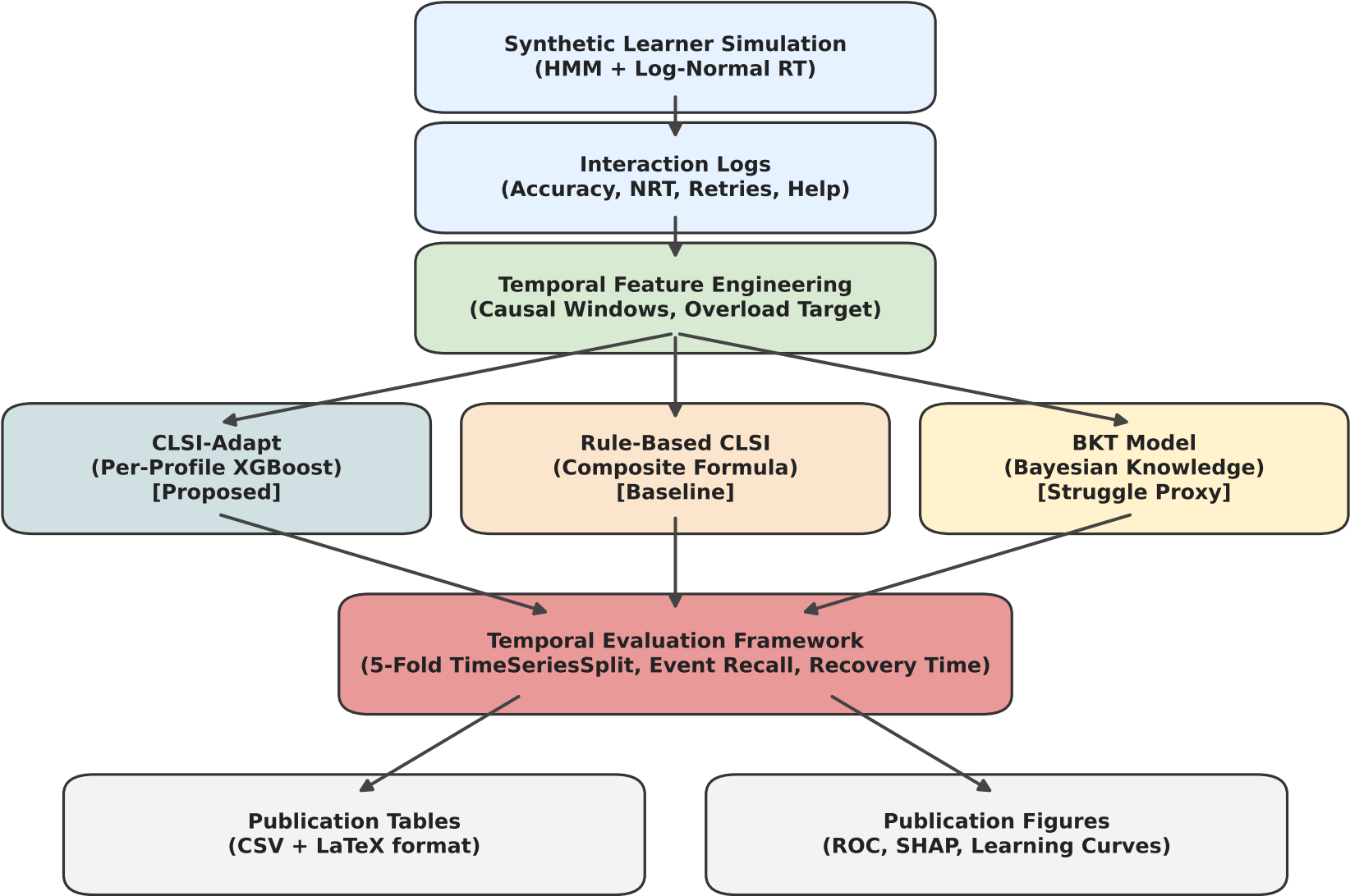
Figure 1: CLSI-Adapt Simulator Architecture & Pipeline Flow
