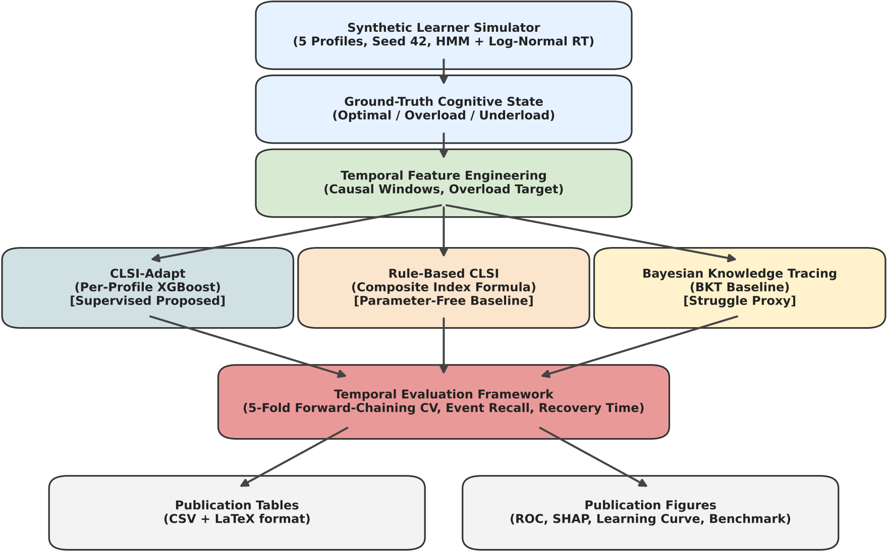
Figure 1: CLSI-Adapt Simulator Architecture & Pipeline Flow
