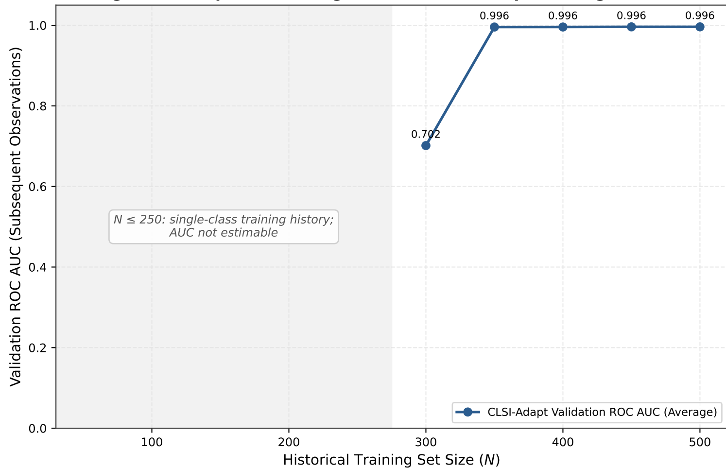
Figure 4. Temporal Learning Curve for CLSI-Adapt (Average Profile)
