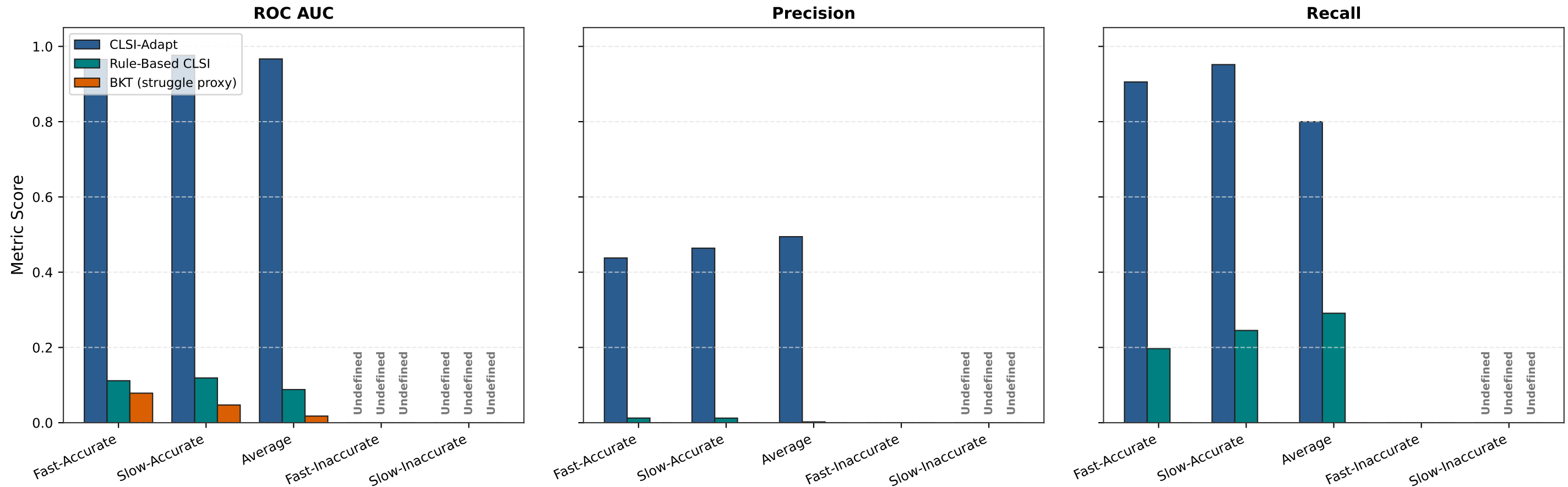
Figure 5. Model Comparison on the Common OOF Evaluation Set
