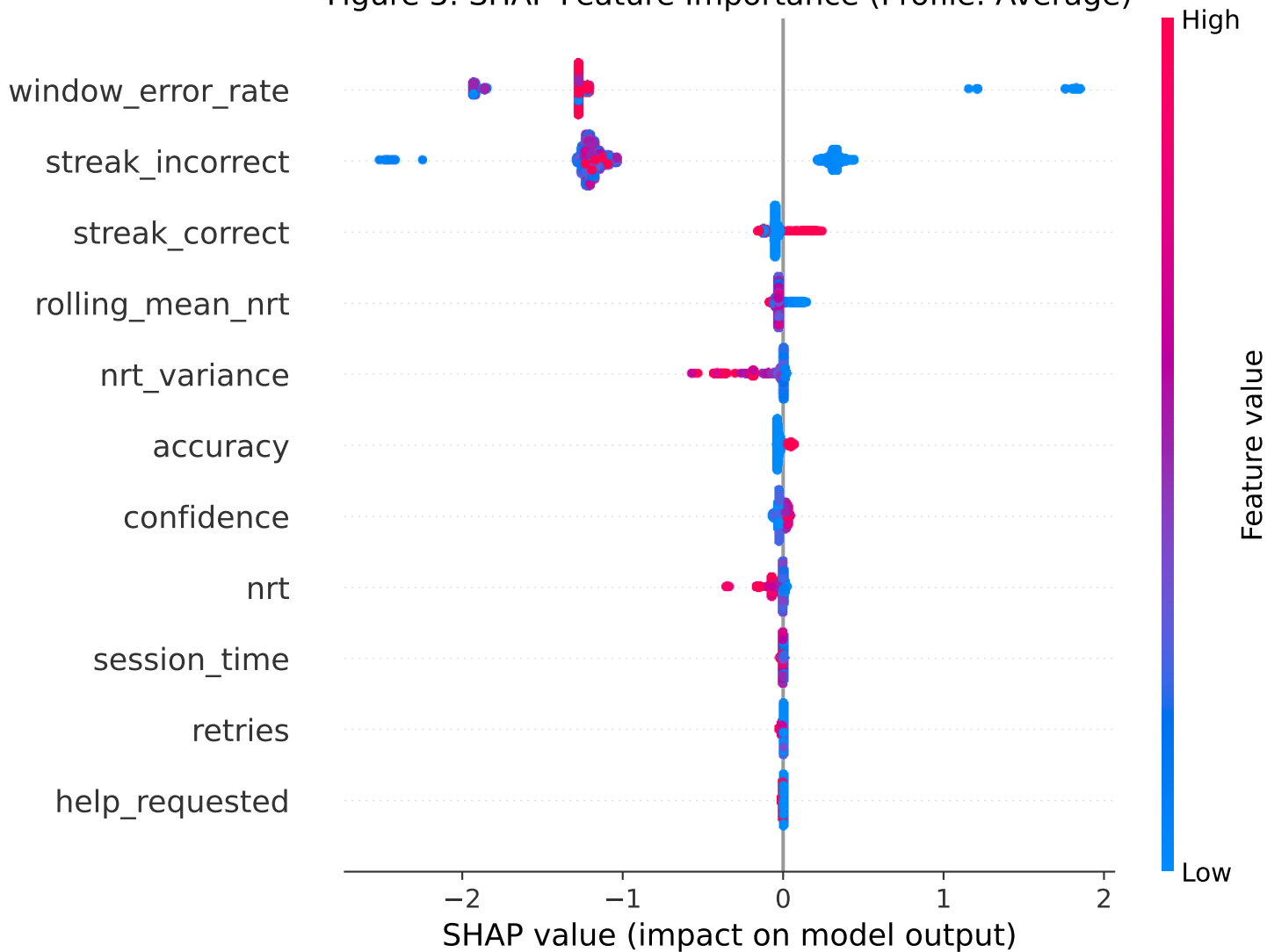
Figure 3: SHAP Feature Importance (Profile: Average)
