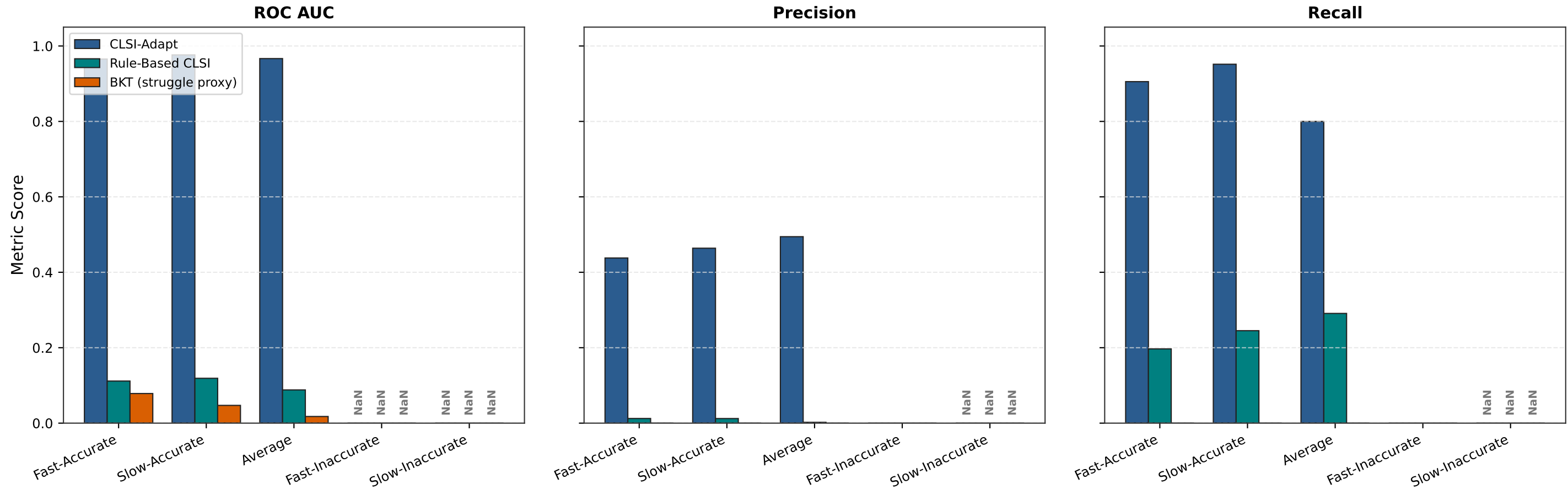
Figure 5: Model Benchmark Comparison Across Learner Profiles (Common OOF Subset)
