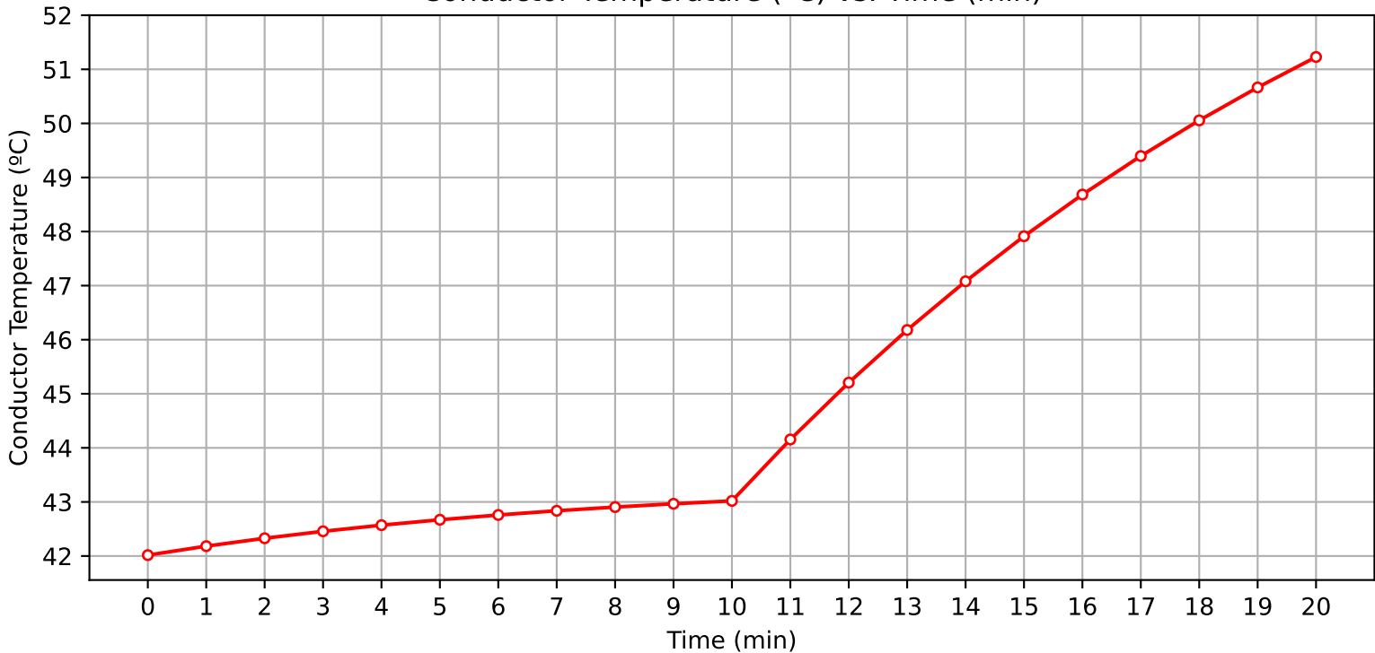
Conductor Temperature ( ^{\circ}\text{C} ) vs. Time (min)
