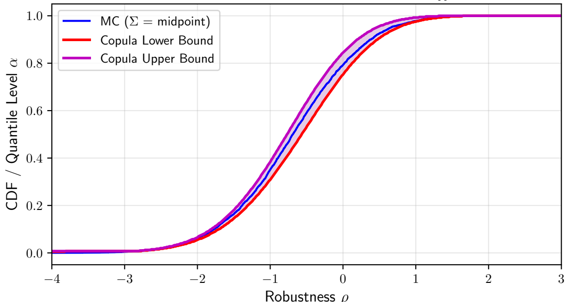
Gaussian: Interval Correlation \Sigma \in [\Sigma_{\text{lower}}, \Sigma_{\text{upper}}]
