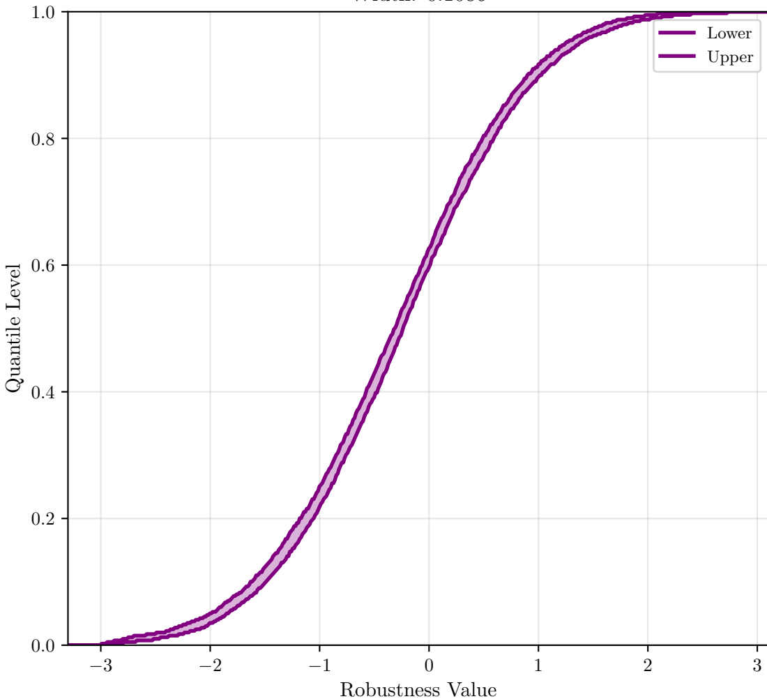
GaussianCopula2D ( \rho = 0.9 , Pairwise) Width: 0.1086
