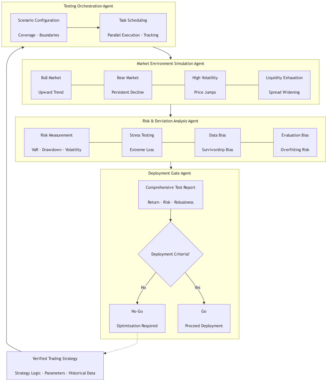
Trading-System Testing MAS
