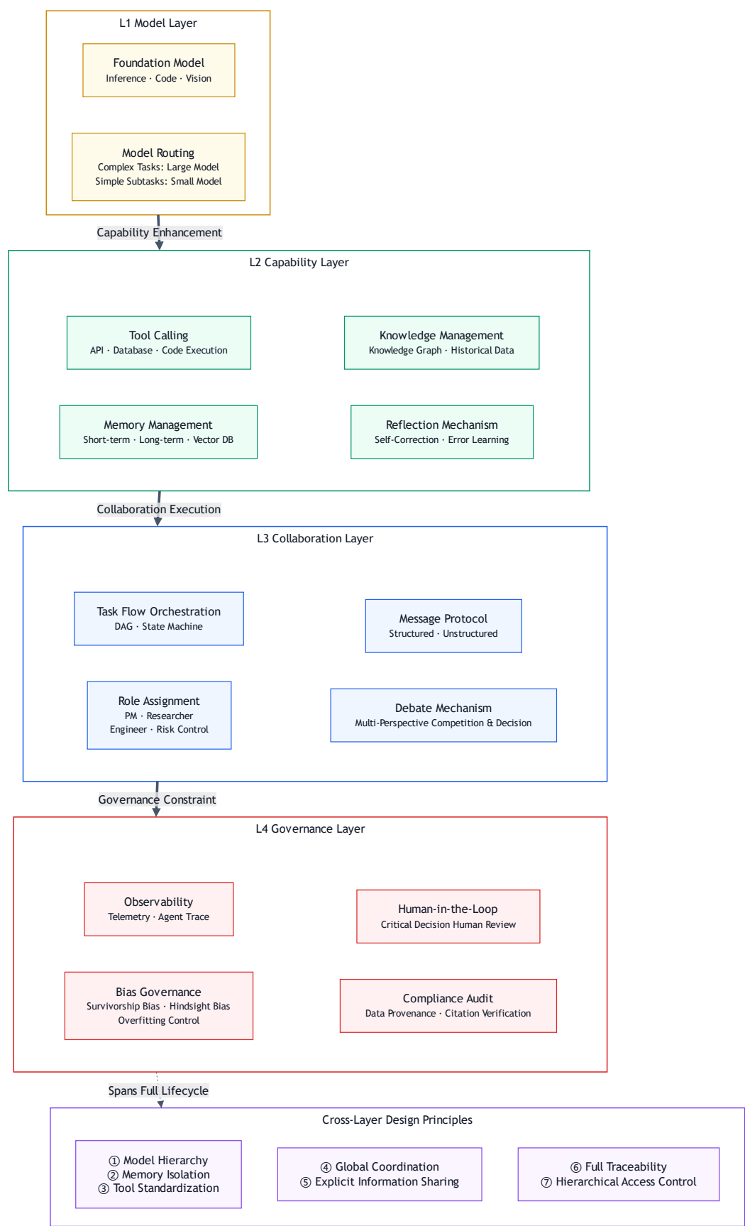
Four-layer reference architecture
