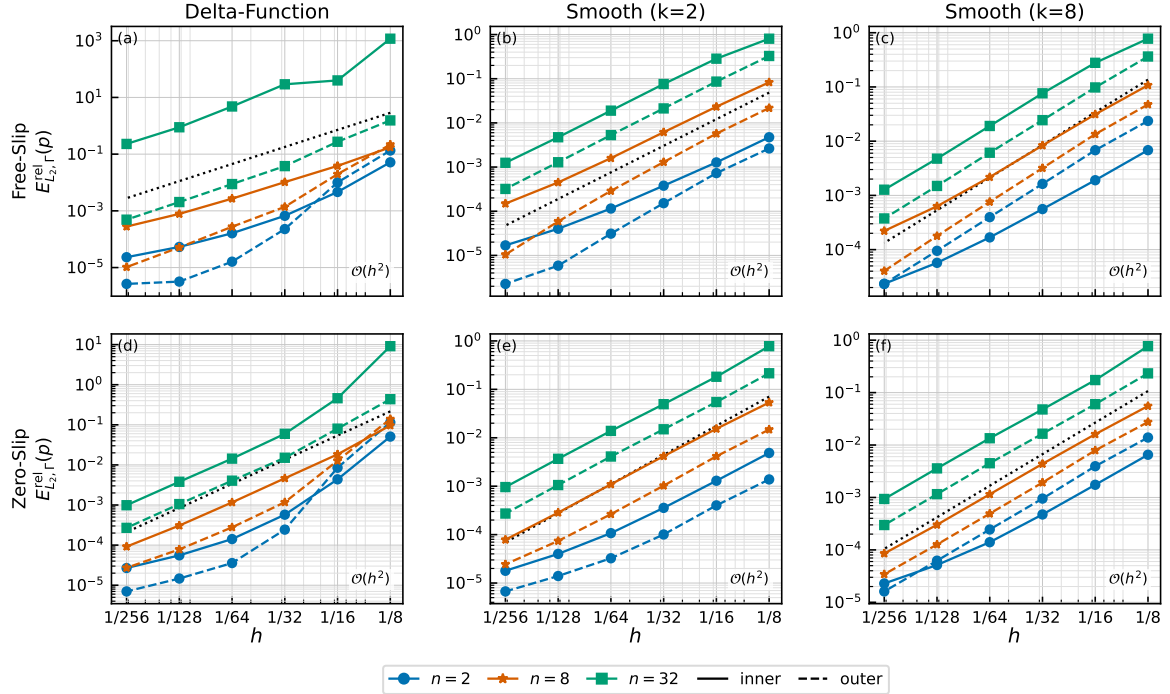
Figure 3. Convergence of relative boundary pressure errors E_{L2,\Gamma}^{\text{rel}}(p) . Solid curves denote the inner boundary and dashed curves denote the outer boundary. Colours indicate azimuthal wavenumber n .
