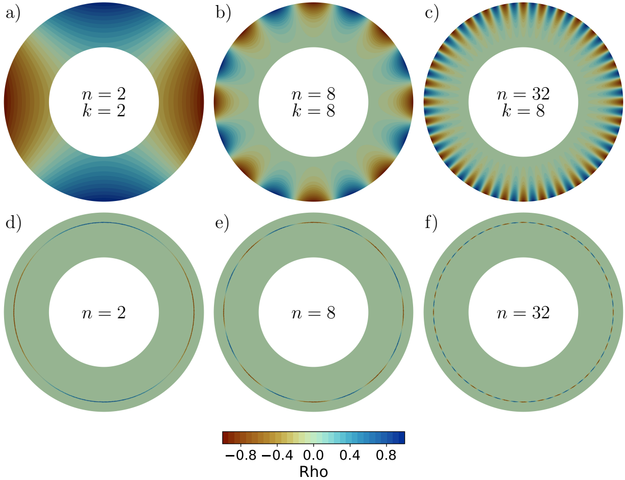
Figure 1. Analytical density perturbations. Panels a)–c) show smooth forcing and panels d)–f) show delta-function forcing. Columns correspond to increasing azimuthal complexity.
