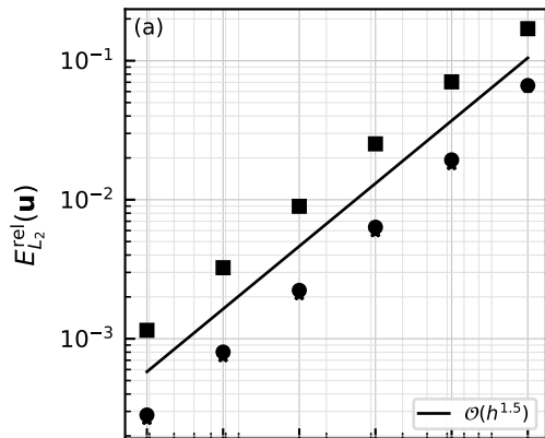
Delta-Function
