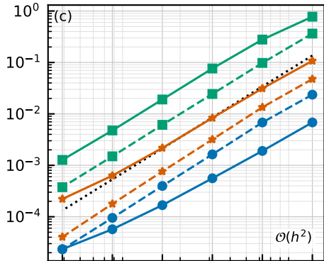
Smooth ( k=8 )
