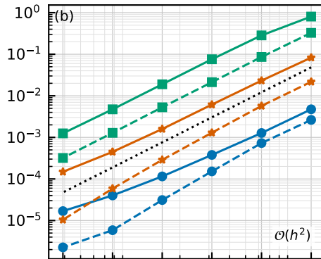
Smooth ( k=2 )
