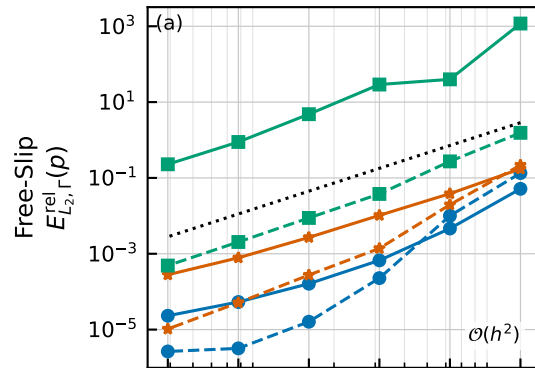
Delta-Function
