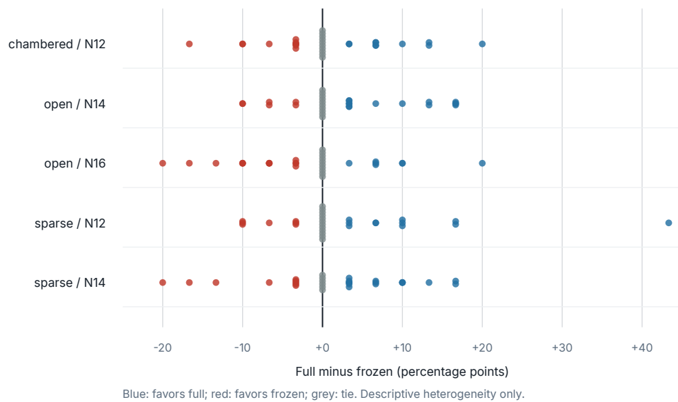
Figure 2: All 150 per-puzzle differences, sorted within stratum. Blue favors full feedback, red favors frozen feedback, and gray is a tie. This plot is descriptive.
