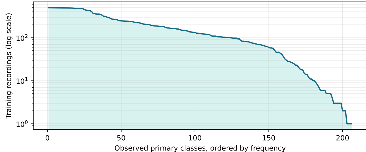
Long-tailed distribution of primary labels
