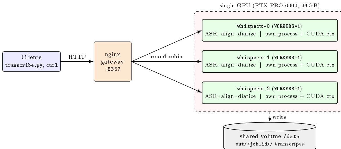
Figure 1: System architecture. Clients issue HTTP to a single nginx gateway (:8357). The gateway round-robins POST /v1/transcribe across the R process replicas and routes each GET /v1/jobs/i-... back to the owning replica i by the numeric job-id prefix, so the process-local job registries need no shared state. Each replica is an independent OS process—its own Python interpreter (hence its own GIL) and CUDA context—running WORKERS=1 with a private ASR/align/diarize model set; all R replicas share one GPU. Finished transcripts are written to a shared /data volume.
