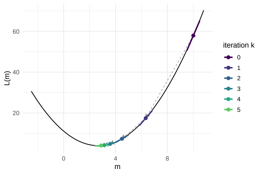
Figure 2.1: The slope idea on the quadratic loss L(m) , for the data of the R run (step size \gamma = 0.25 , chosen to make a clean picture). Each coloured point is an iterate m_k , and the short segment through it shows the local slope there: the slope points uphill, so the update steps the other way (dashed arrows), and as the slope flattens towards the minimum the steps shrink on their own.
